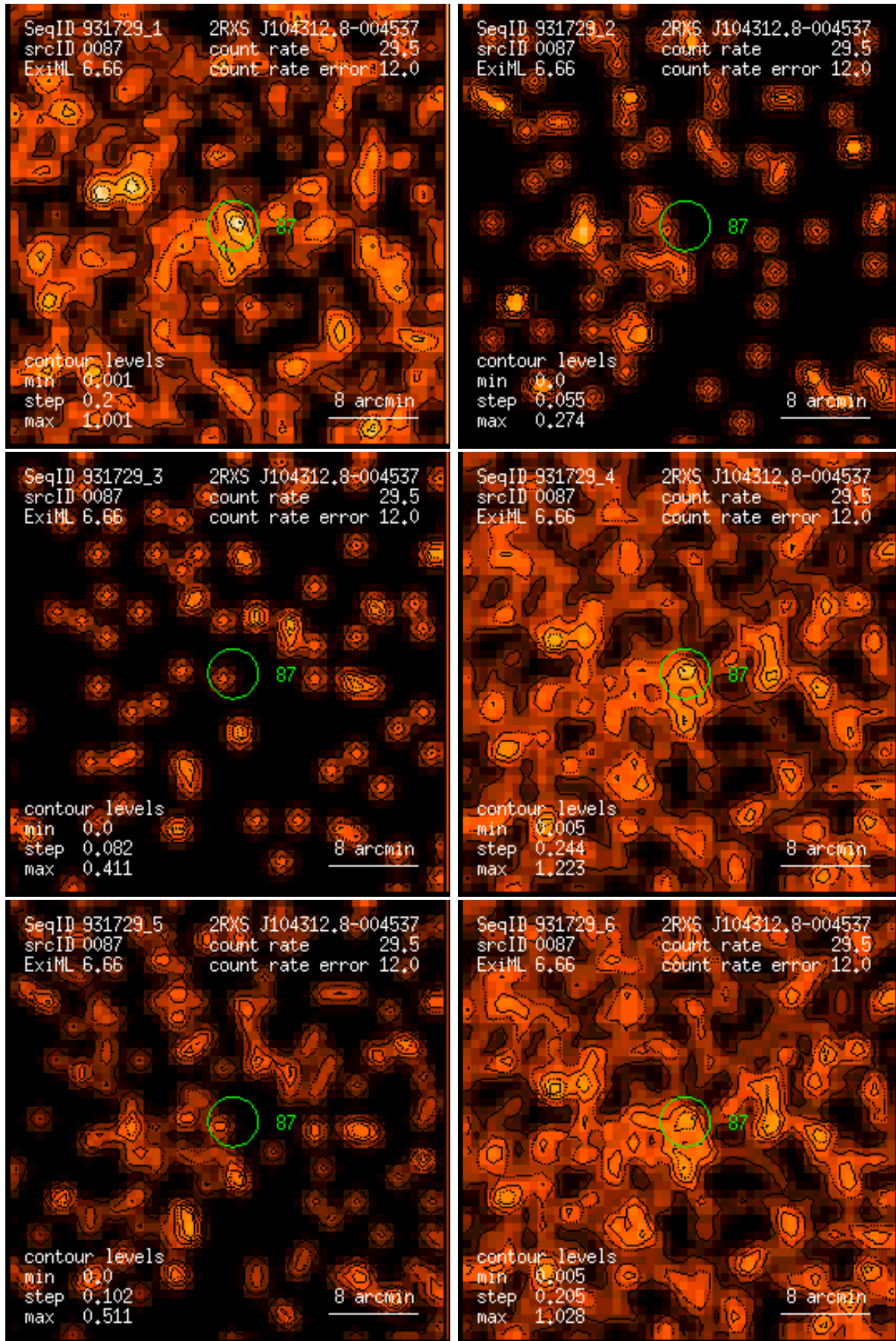
Figure 87: RASS 931729: detection 0087: band rate images, Gaussian filter: (1) PSPC channels 11 – 41, (2) 52 – 90, (3) 91 – 201, (4) 11 – 235, (5) 52 – 201, (6) 11 – 201. Broad band rates in counts/ks. Band rate contour levels in counts/ks/arcmin 2 .
