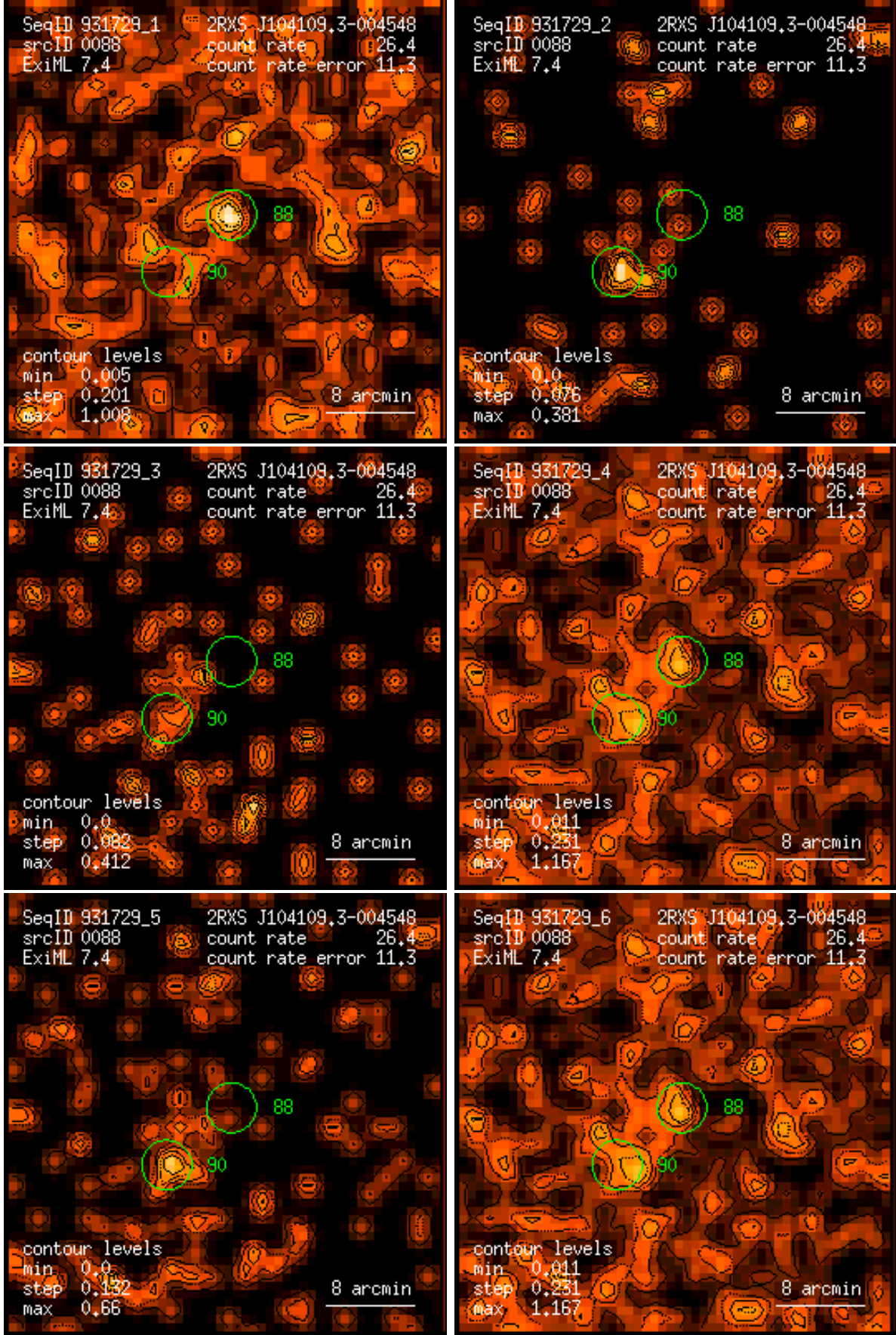
Figure 88: RASS 931729: detection 0088: band rate images, Gaussian filter: (1) PSPC channels 11 – 41, (2) 52 – 90, (3) 91 – 201, (4) 11 – 235, (5) 52 – 201, (6) 11 – 201. Broad band rates in counts/ks. Band rate contour levels in counts/ks/arcmin 2 .
