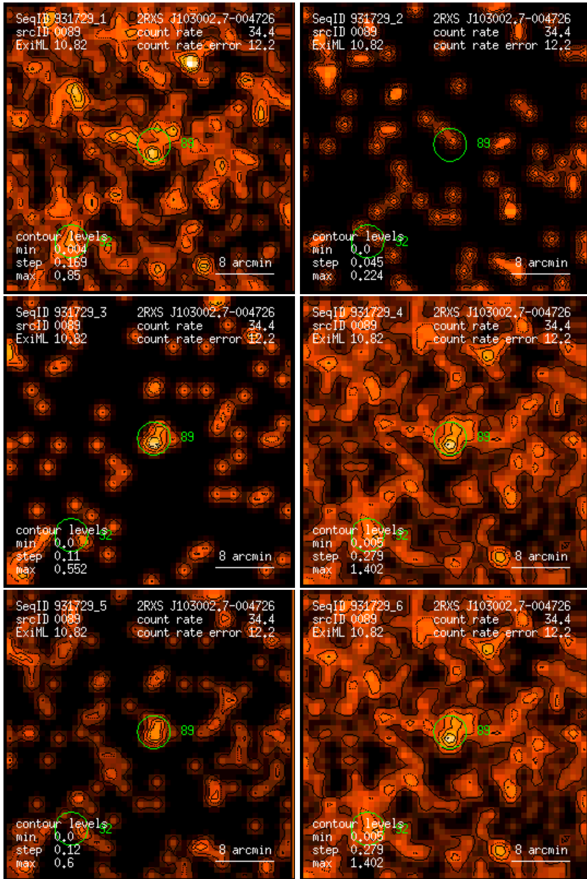
Figure 89: RASS 931729: detection 0089: band rate images, Gaussian filter: (1) PSPC channels 11 – 41, (2) 52 – 90, (3) 91 – 201, (4) 11 – 235, (5) 52 – 201, (6) 11 – 201. Broad band rates in counts/ks. Band rate contour levels in counts/ks/arcmin 2 .
