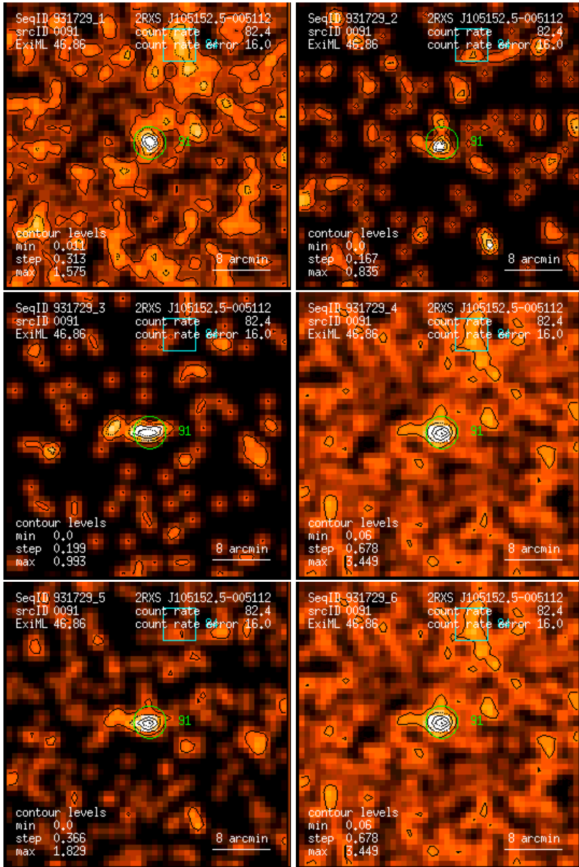
Figure 91: RASS 931729: detection 0091: band rate images, Gaussian filter: (1) PSPC channels 11 – 41, (2) 52 – 90, (3) 91 – 201, (4) 11 – 235, (5) 52 – 201, (6) 11 – 201. Broad band rates in counts/ks. Band rate contour levels in counts/ks/arcmin 2 .
