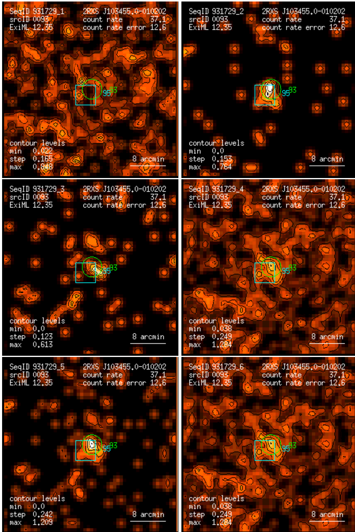
Figure 93: RASS 931729: detection 0093: band rate images, Gaussian filter: (1) PSPC channels 11 – 41, (2) 52 – 90, (3) 91 – 201, (4) 11 – 235, (5) 52 – 201, (6) 11 – 201. Broad band rates in counts/ks. Band rate contour levels in counts/ks/arcmin 2 .
