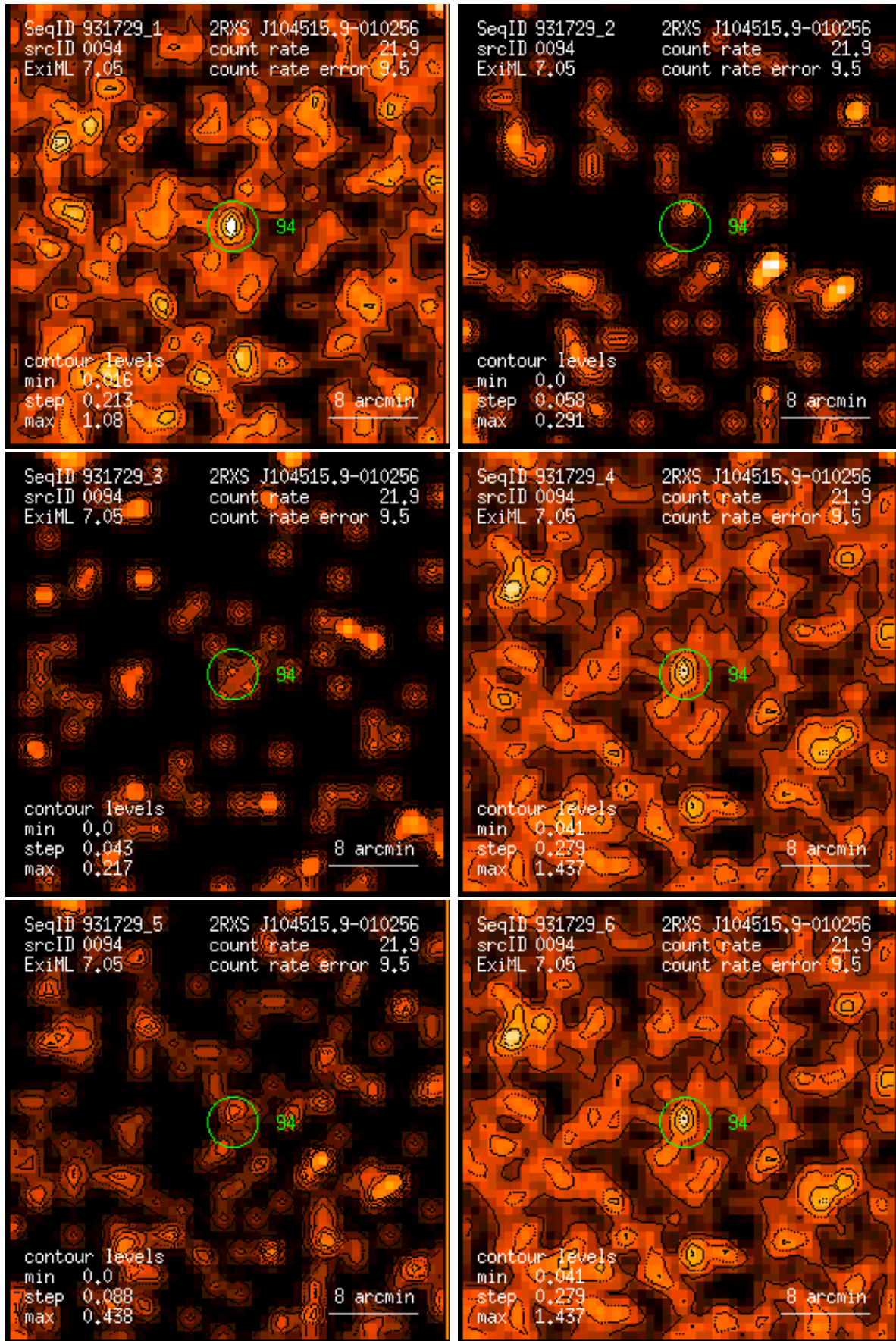
Figure 94: RASS 931729: detection 0094: band rate images, Gaussian filter: (1) PSPC channels 11 – 41, (2) 52 – 90, (3) 91 – 201, (4) 11 – 235, (5) 52 – 201, (6) 11 – 201. Broad band rates in counts/ks. Band rate contour levels in counts/ks/arcmin 2 .
