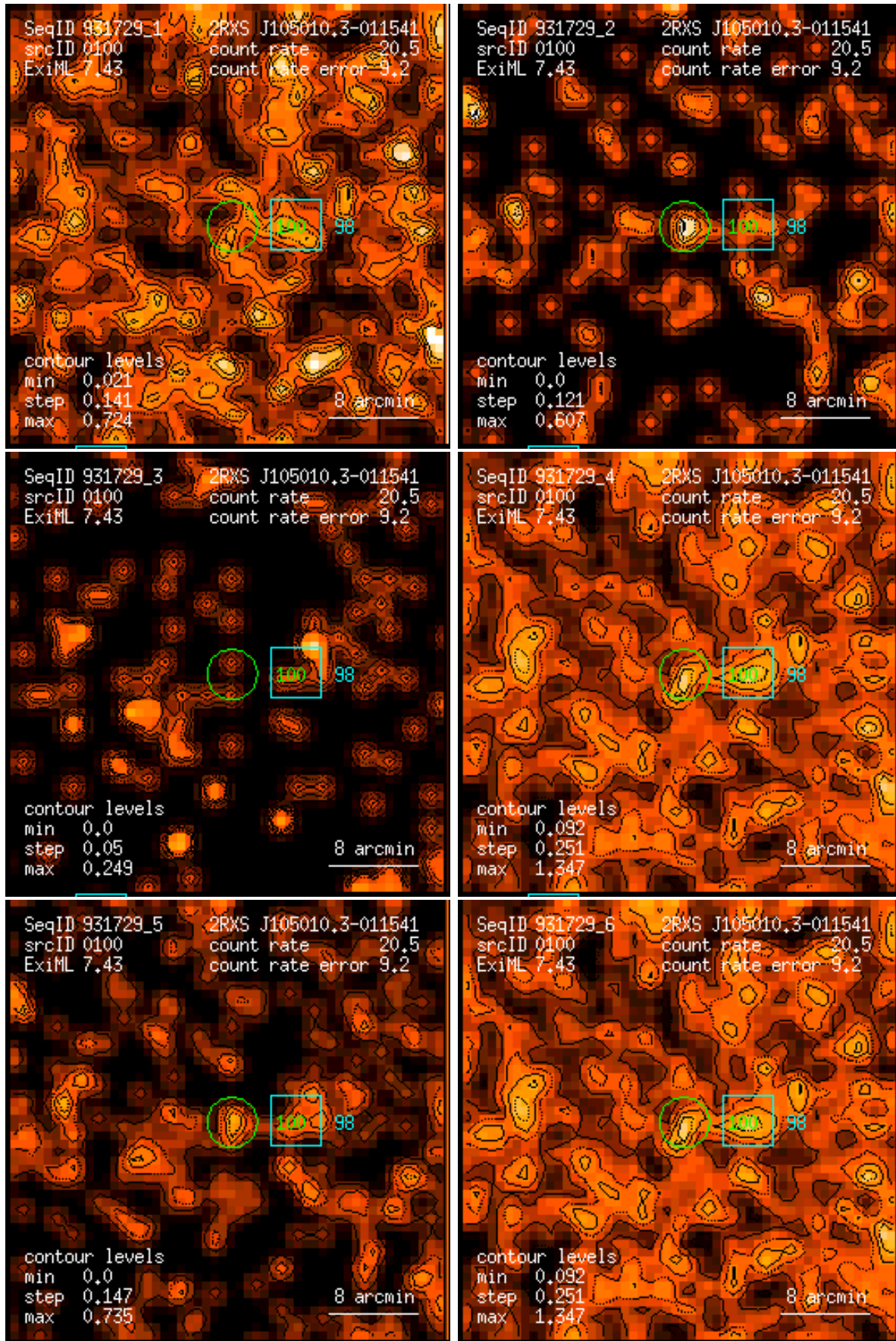
Figure 100: RASS 931729: detection 0100: band rate images, Gaussian filter: (1) PSPC channels 11 – 41, (2) 52 – 90, (3) 91 – 201, (4) 11 – 235, (5) 52 – 201, (6) 11 – 201. Broad band rates in counts/ks. Band rate contour levels in counts/ks/arcmin 2 .
