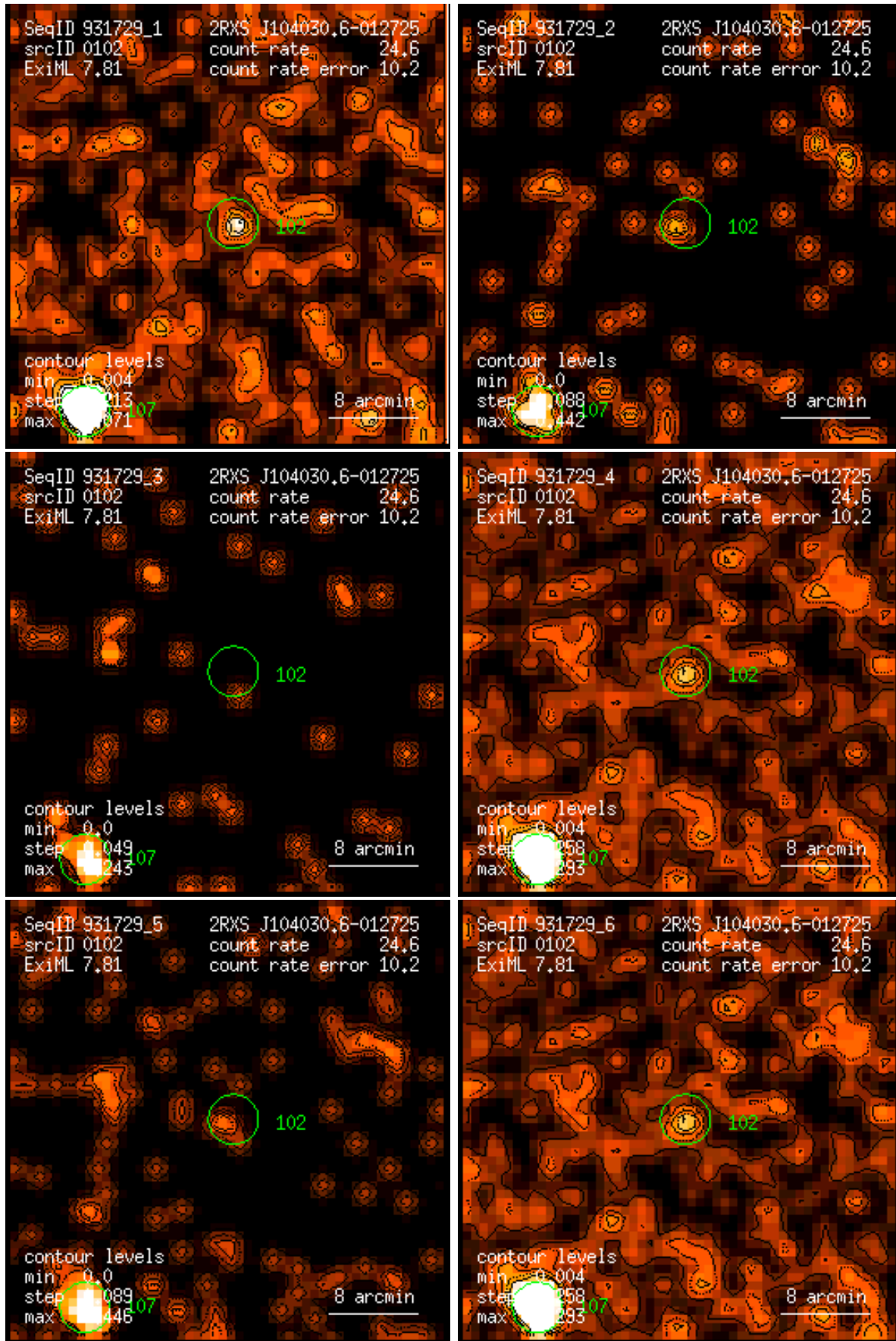
Figure 102: RASS 931729: detection 0102: band rate images, Gaussian filter: (1) PSPC channels 11 – 41, (2) 52 – 90, (3) 91 – 201, (4) 11 – 235, (5) 52 – 201, (6) 11 – 201. Broad band rates in counts/ks. Band rate contour levels in counts/ks/arcmin 2 .
