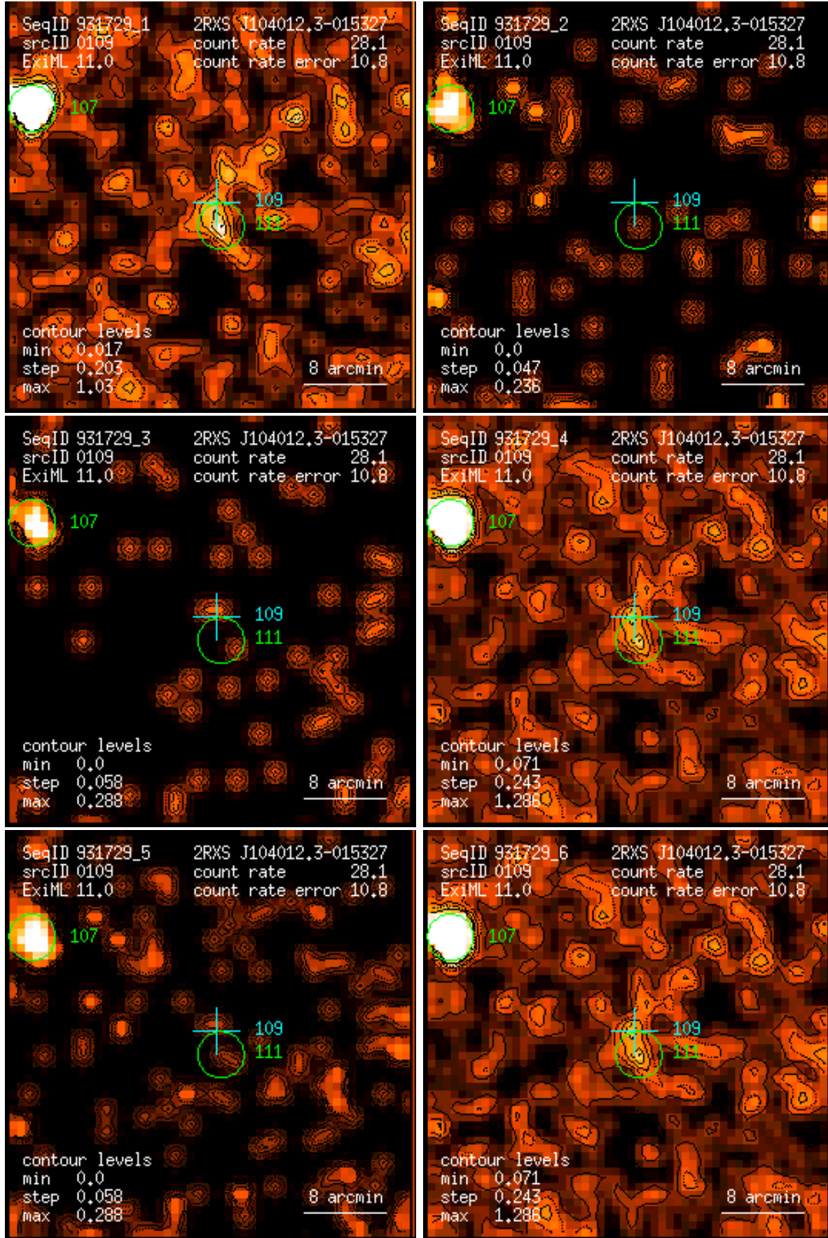
Figure 109: RASS 931729: detection 0109: band rate images, Gaussian filter: (1) PSPC channels 11 – 41, (2) 52 – 90, (3) 91 – 201, (4) 11 – 235, (5) 52 – 201, (6) 11 – 201. Broad band rates in counts/ks. Band rate contour levels in counts/ks/arcmin 2 .
