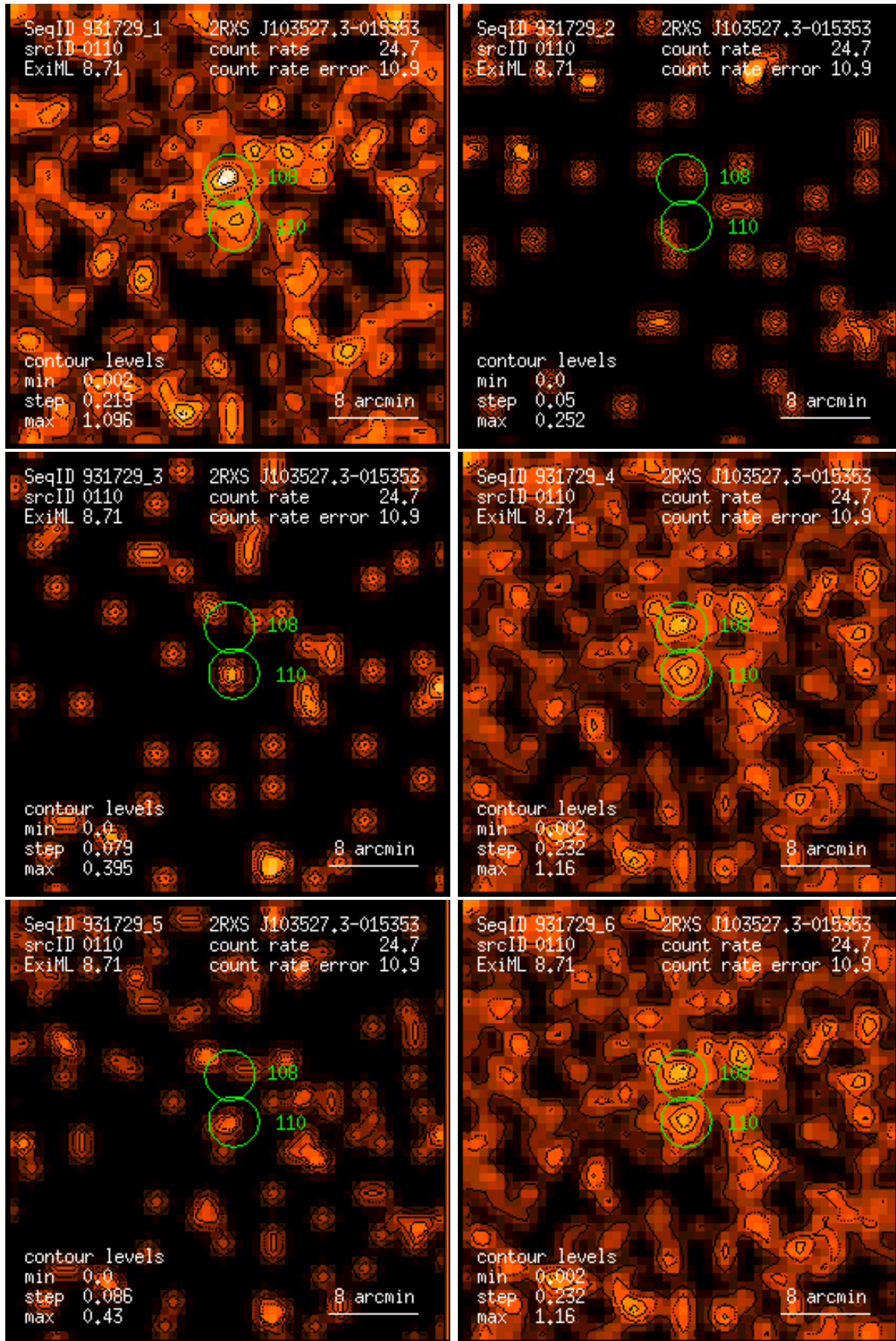
Figure 110: RASS 931729: detection 0110: band rate images, Gaussian filter: (1) PSPC channels 11 – 41, (2) 52 – 90, (3) 91 – 201, (4) 11 – 235, (5) 52 – 201, (6) 11 – 201. Broad band rates in counts/ks. Band rate contour levels in counts/ks/arcmin 2 .
