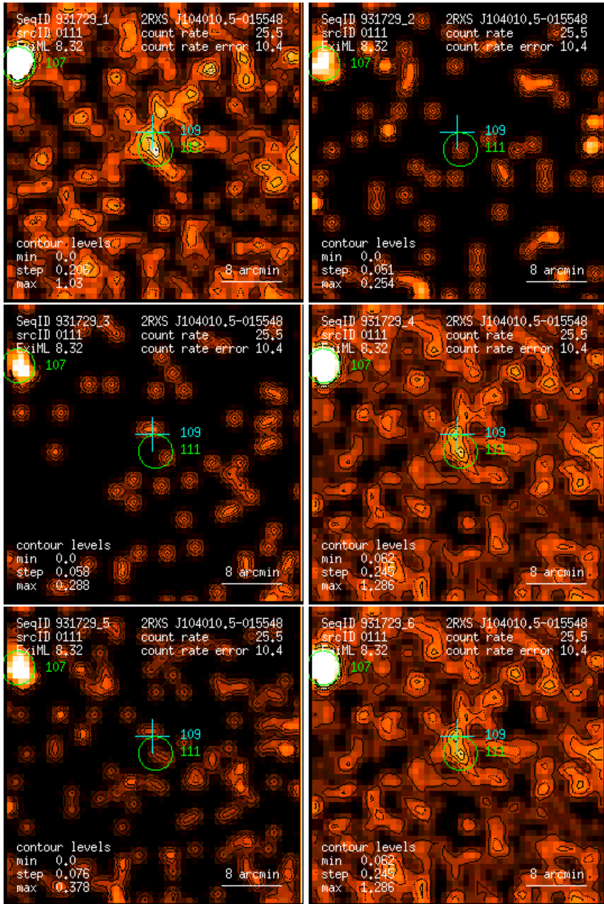
Figure 111: RASS 931729: detection 0111: band rate images, Gaussian filter: (1) PSPC channels 11 – 41, (2) 52 – 90, (3) 91 – 201, (4) 11 – 235, (5) 52 – 201, (6) 11 – 201. Broad band rates in counts/ks. Band rate contour levels in counts/ks/arcmin 2 .
