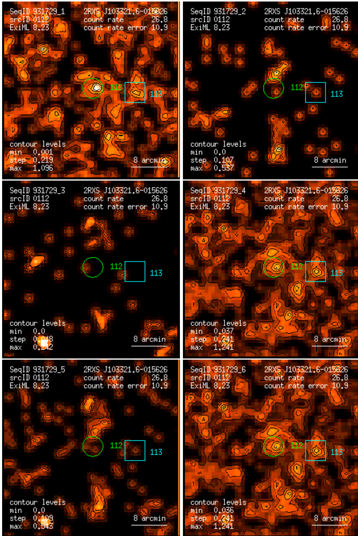
Figure 112: RASS 931729: detection 0112: band rate images, Gaussian filter: (1) PSPC channels 11 – 41, (2) 52 – 90, (3) 91 – 201, (4) 11 – 235, (5) 52 – 201, (6) 11 – 201. Broad band rates in counts/ks. Band rate contour levels in counts/ks/arcmin 2 .
