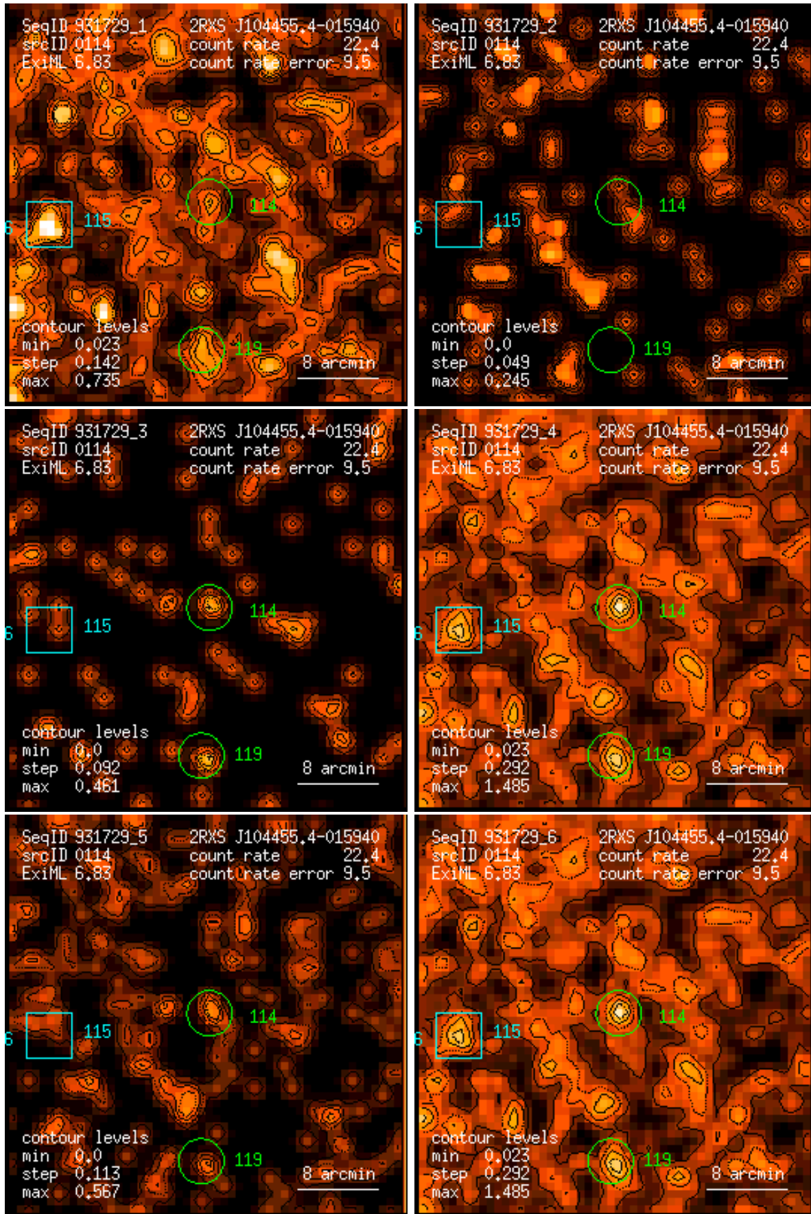
Figure 114: RASS 931729: detection 0114: band rate images, Gaussian filter: (1) PSPC channels 11 – 41, (2) 52 – 90, (3) 91 – 201, (4) 11 – 235, (5) 52 – 201, (6) 11 – 201. Broad band rates in counts/ks. Band rate contour levels in counts/ks/arcmin 2 .
