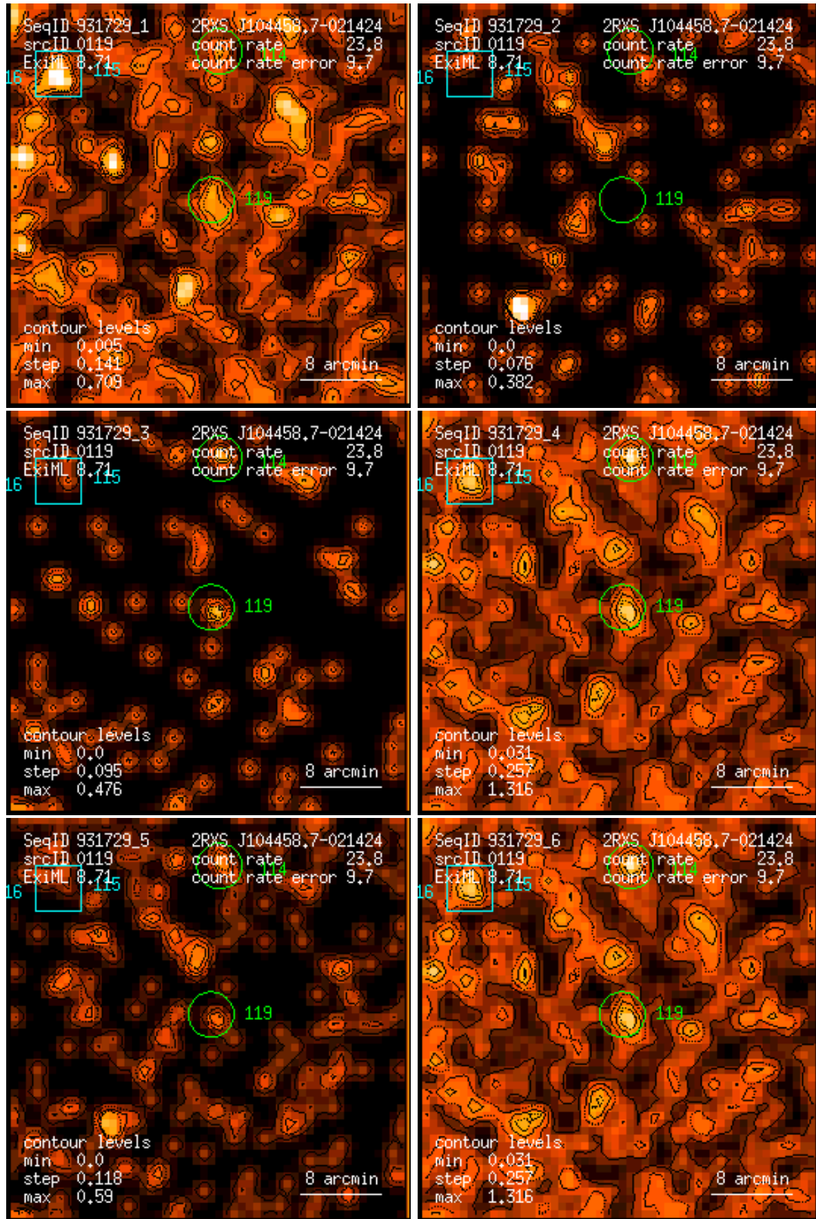
Figure 119: RASS 931729: detection 0119: band rate images, Gaussian filter: (1) PSPC channels 11 – 41, (2) 52 – 90, (3) 91 – 201, (4) 11 – 235, (5) 52 – 201, (6) 11 – 201. Broad band rates in counts/ks. Band rate contour levels in counts/ks/arcmin 2 .
