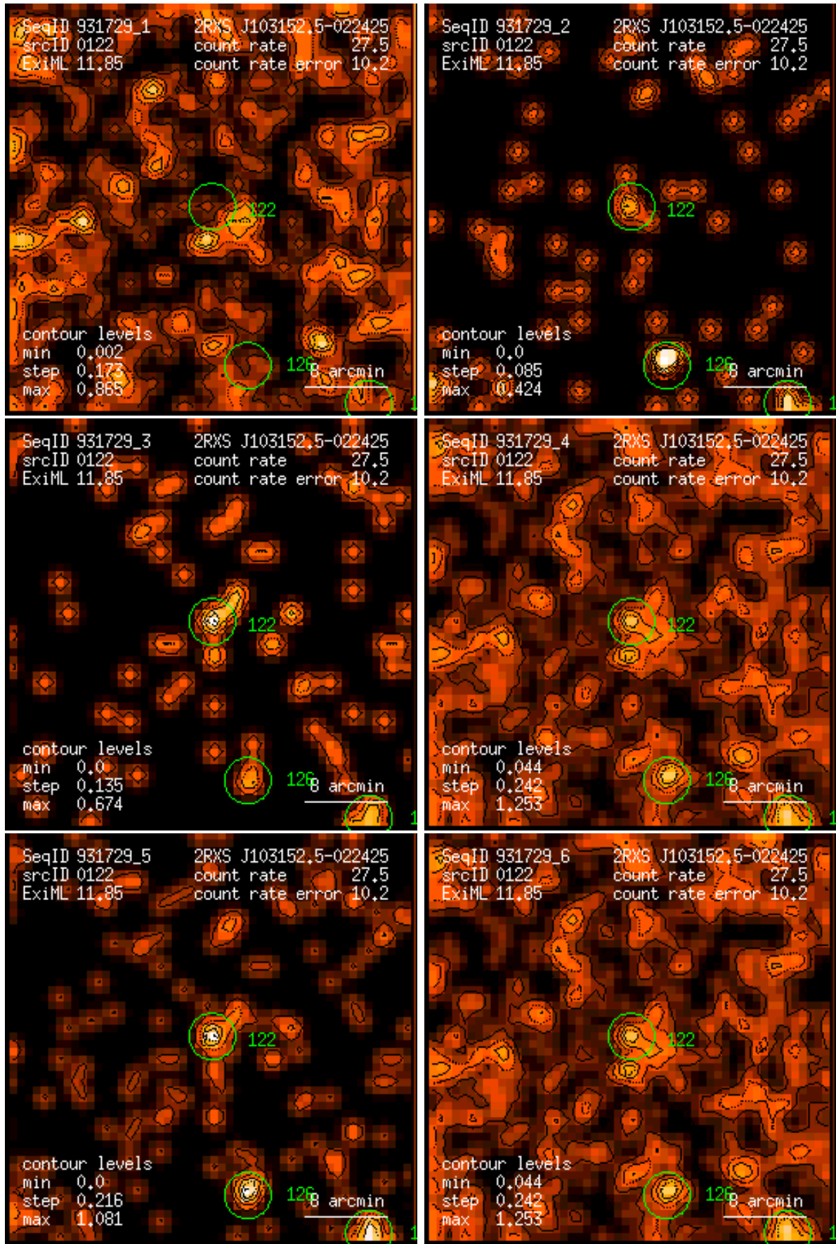
Figure 122: RASS 931729: detection 0122: band rate images, Gaussian filter: (1) PSPC channels 11 – 41, (2) 52 – 90, (3) 91 – 201, (4) 11 – 235, (5) 52 – 201, (6) 11 – 201. Broad band rates in counts/ks. Band rate contour levels in counts/ks/arcmin 2 .
