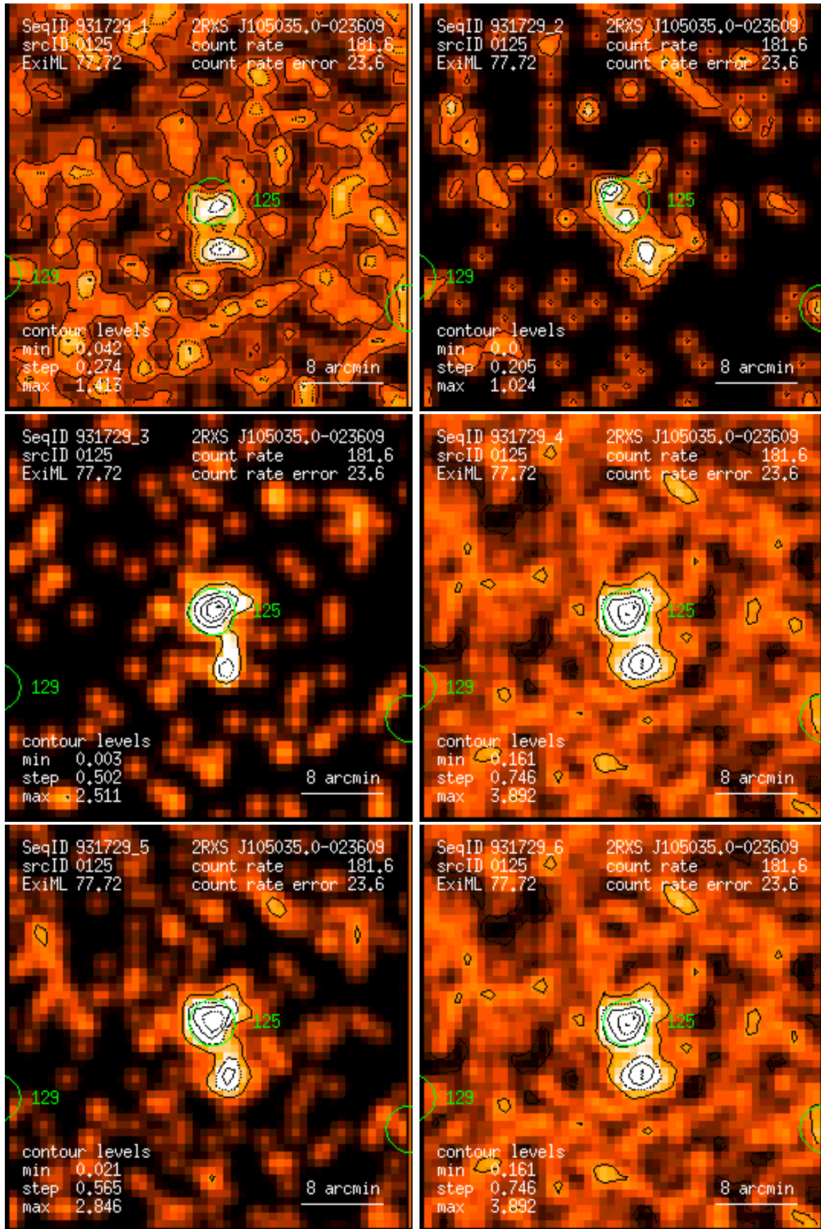
Figure 125: RASS 931729: detection 0125: band rate images, Gaussian filter: (1) PSPC channels 11 – 41, (2) 52 – 90, (3) 91 – 201, (4) 11 – 235, (5) 52 – 201, (6) 11 – 201. Broad band rates in counts/ks. Band rate contour levels in counts/ks/arcmin 2 .
