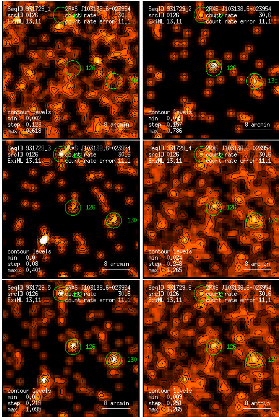
Figure 126: RASS 931729: detection 0126: band rate images, Gaussian filter: (1) PSPC channels 11 – 41, (2) 52 – 90, (3) 91 – 201, (4) 11 – 235, (5) 52 – 201, (6) 11 – 201. Broad band rates in counts/ks. Band rate contour levels in counts/ks/arcmin 2 .
