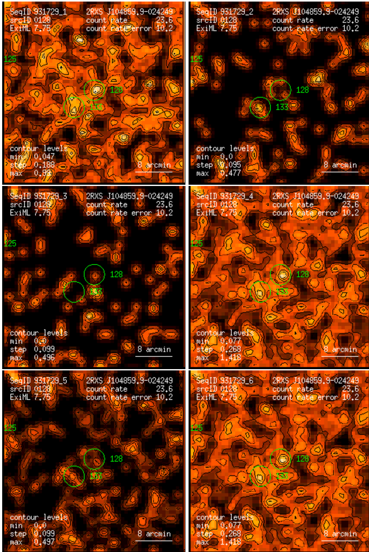
Figure 128: RASS 931729: detection 0128: band rate images, Gaussian filter: (1) PSPC channels 11 – 41, (2) 52 – 90, (3) 91 – 201, (4) 11 – 235, (5) 52 – 201, (6) 11 – 201. Broad band rates in counts/ks. Band rate contour levels in counts/ks/arcmin 2 .
