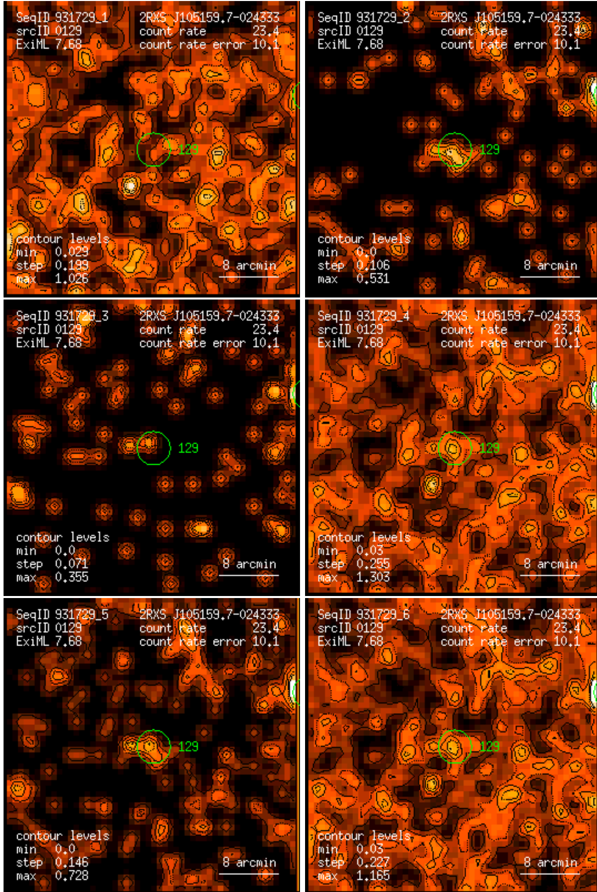
Figure 129: RASS 931729: detection 0129: band rate images, Gaussian filter: (1) PSPC channels 11 – 41, (2) 52 – 90, (3) 91 – 201, (4) 11 – 235, (5) 52 – 201, (6) 11 – 201. Broad band rates in counts/ks. Band rate contour levels in counts/ks/arcmin 2 .
