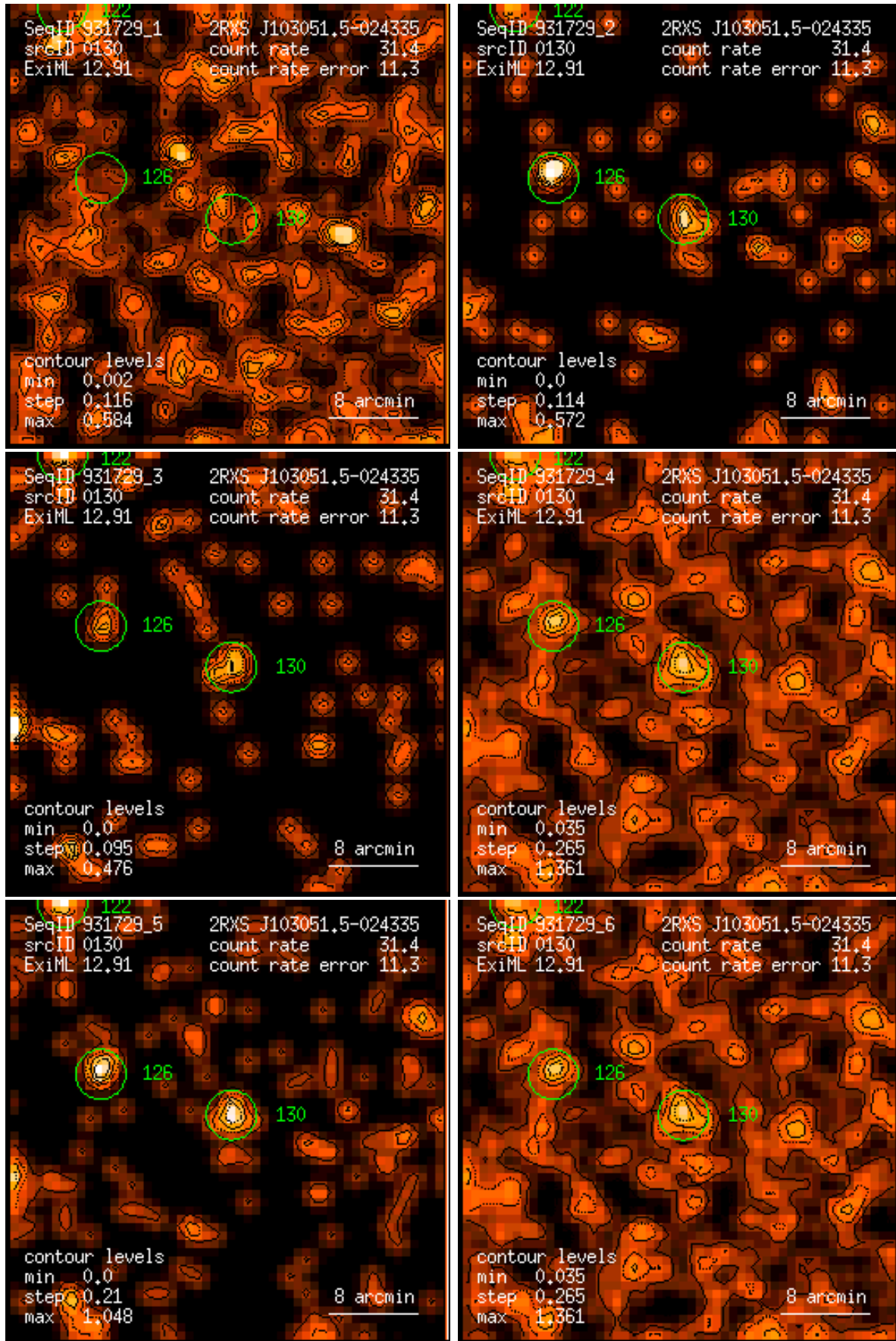
Figure 130: RASS 931729: detection 0130: band rate images, Gaussian filter: (1) PSPC channels 11 – 41, (2) 52 – 90, (3) 91 – 201, (4) 11 – 235, (5) 52 – 201, (6) 11 – 201. Broad band rates in counts/ks. Band rate contour levels in counts/ks/arcmin 2 .
