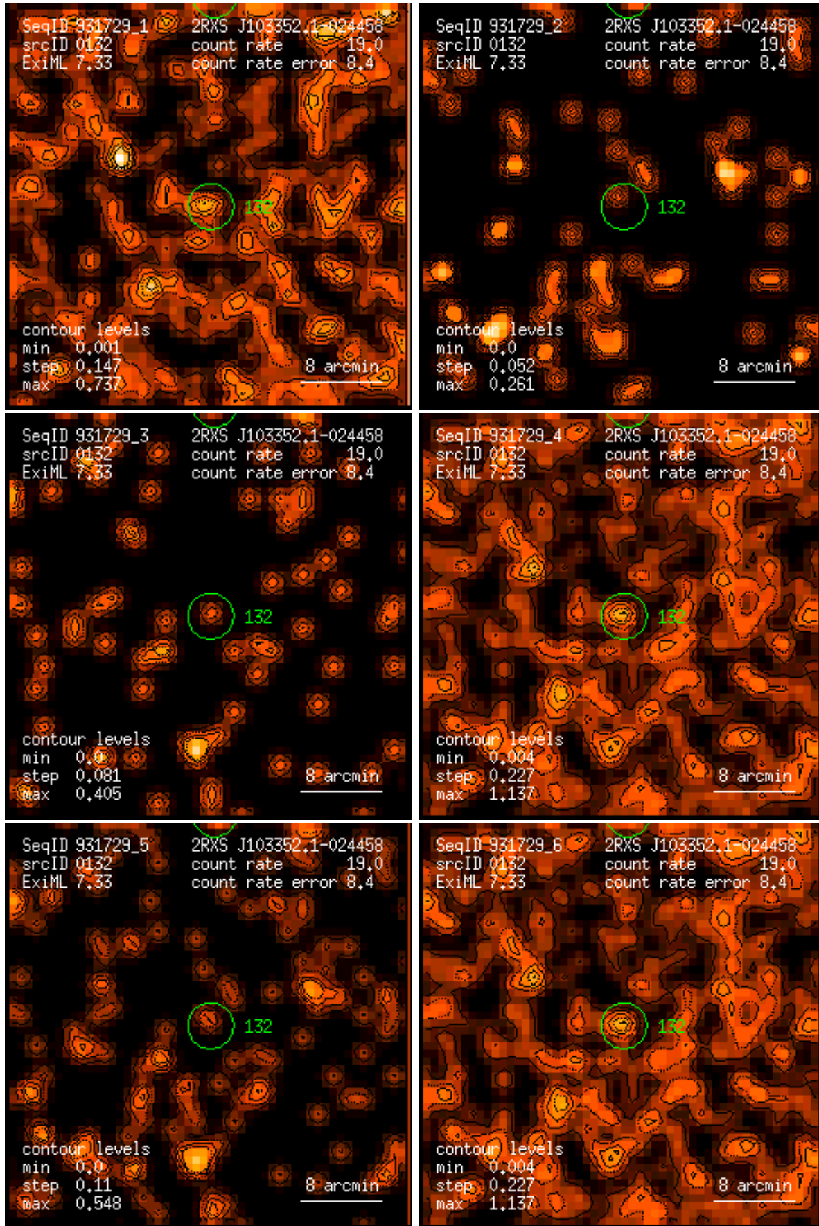
Figure 132: RASS 931729: detection 0132: band rate images, Gaussian filter: (1) PSPC channels 11 – 41, (2) 52 – 90, (3) 91 – 201, (4) 11 – 235, (5) 52 – 201, (6) 11 – 201. Broad band rates in counts/ks. Band rate contour levels in counts/ks/arcmin 2 .
