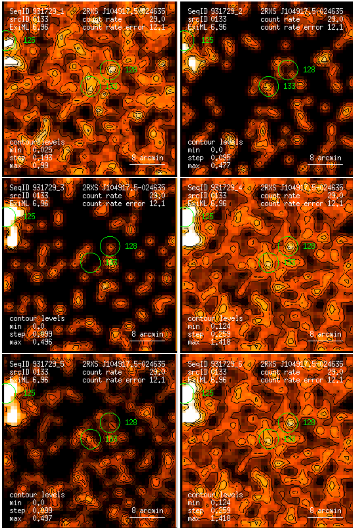
Figure 133: RASS 931729: detection 0133: band rate images, Gaussian filter: (1) PSPC channels 11 – 41, (2) 52 – 90, (3) 91 – 201, (4) 11 – 235, (5) 52 – 201, (6) 11 – 201. Broad band rates in counts/ks. Band rate contour levels in counts/ks/arcmin 2 .
