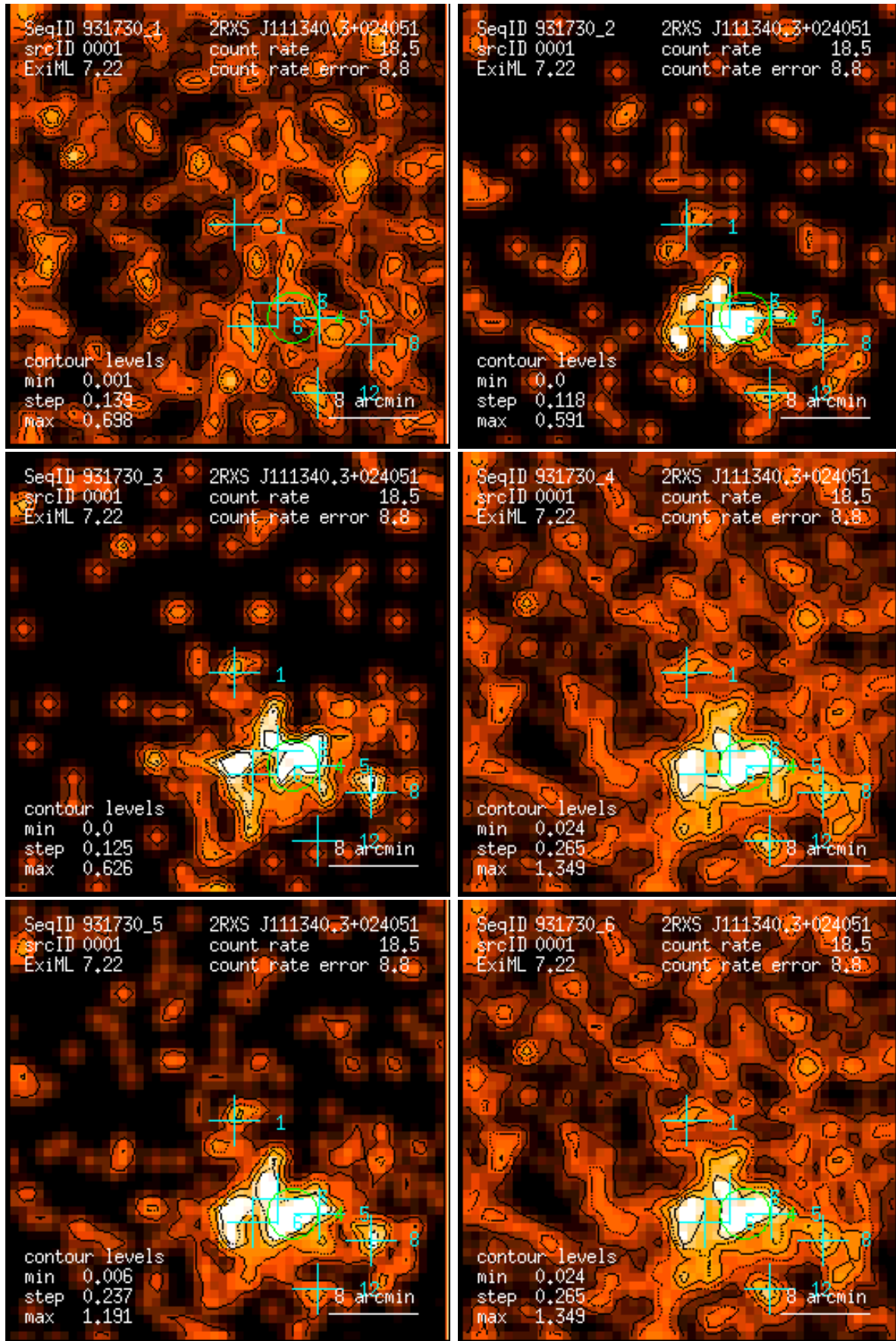
Figure 1: RASS 931730: detection 0001: band rate images, Gaussian filter: (1) PSPC channels 11 – 41, (2) 52 – 90, (3) 91 – 201, (4) 11 – 235, (5) 52 – 201, (6) 11 – 201. Broad band rates in counts/ks. Band rate contour levels in counts/ks/arcmin 2 .
