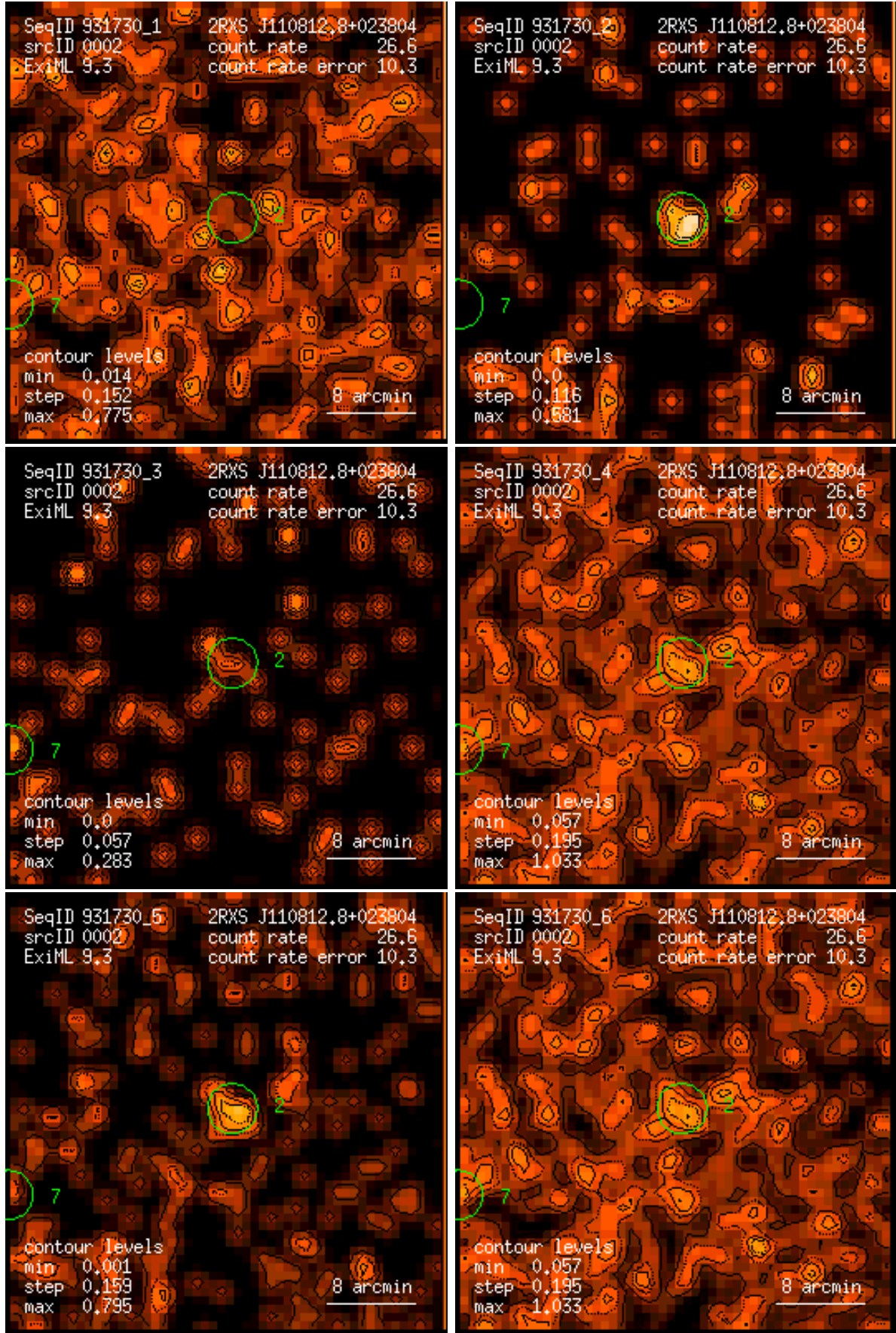
Figure 2: RASS 931730: detection 0002: band rate images, Gaussian filter: (1) PSPC channels 11 – 41, (2) 52 – 90, (3) 91 – 201, (4) 11 – 235, (5) 52 – 201, (6) 11 – 201. Broad band rates in counts/ks. Band rate contour levels in counts/ks/arcmin 2 .
