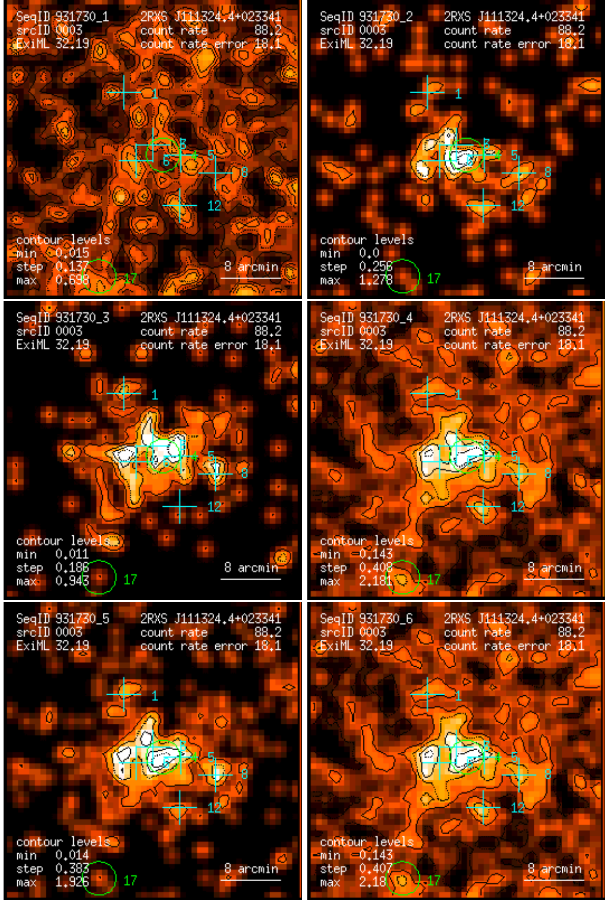
Figure 3: RASS 931730: detection 0003: band rate images, Gaussian filter: (1) PSPC channels 11 – 41, (2) 52 – 90, (3) 91 – 201, (4) 11 – 235, (5) 52 – 201, (6) 11 – 201. Broad band rates in counts/ks. Band rate contour levels in counts/ks/arcmin 2 .
