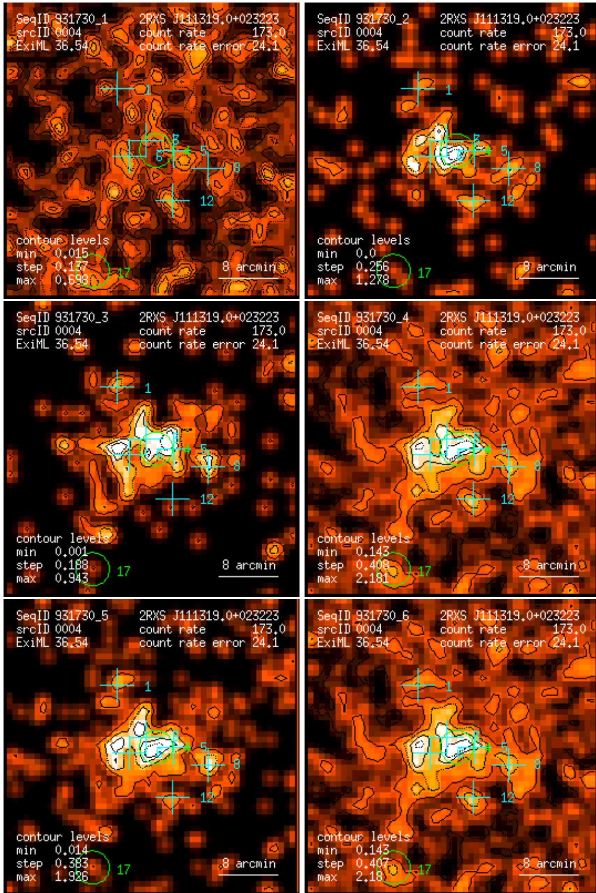
Figure 4: RASS 931730: detection 0004: band rate images, Gaussian filter: (1) PSPC channels 11 – 41, (2) 52 – 90, (3) 91 – 201, (4) 11 – 235, (5) 52 – 201, (6) 11 – 201. Broad band rates in counts/ks. Band rate contour levels in counts/ks/arcmin 2 .
