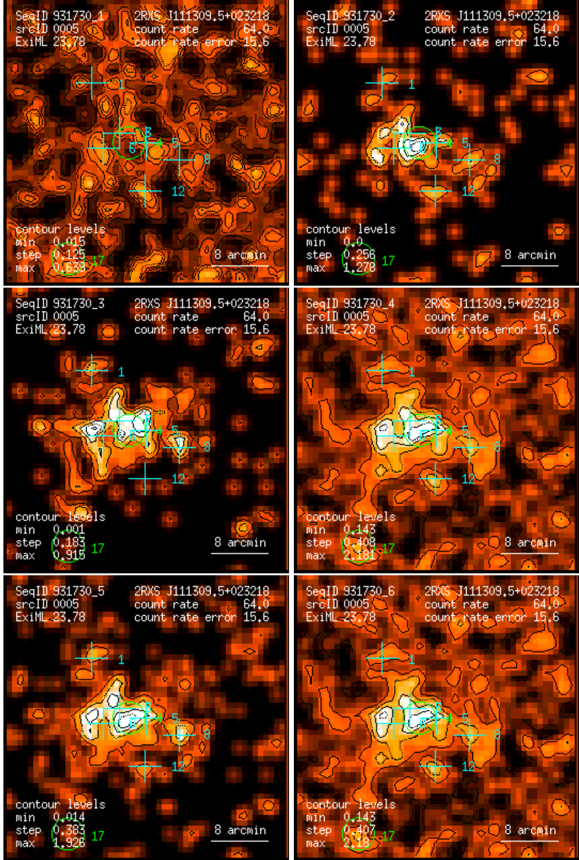
Figure 5: RASS 931730: detection 0005: band rate images, Gaussian filter: (1) PSPC channels 11 – 41, (2) 52 – 90, (3) 91 – 201, (4) 11 – 235, (5) 52 – 201, (6) 11 – 201. Broad band rates in counts/ks. Band rate contour levels in counts/ks/arcmin 2 .
