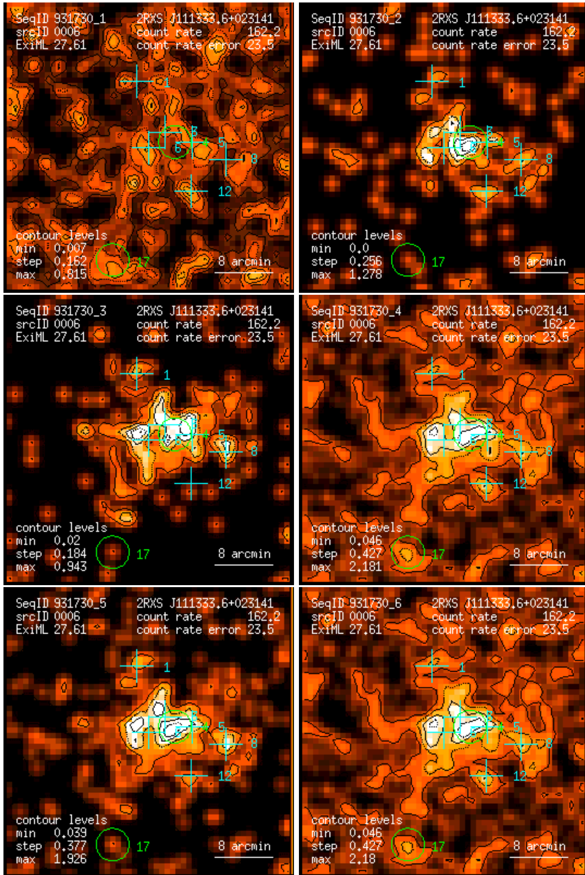
Figure 6: RASS 931730: detection 0006: band rate images, Gaussian filter: (1) PSPC channels 11 – 41, (2) 52 – 90, (3) 91 – 201, (4) 11 – 235, (5) 52 – 201, (6) 11 – 201. Broad band rates in counts/ks. Band rate contour levels in counts/ks/arcmin 2 .
