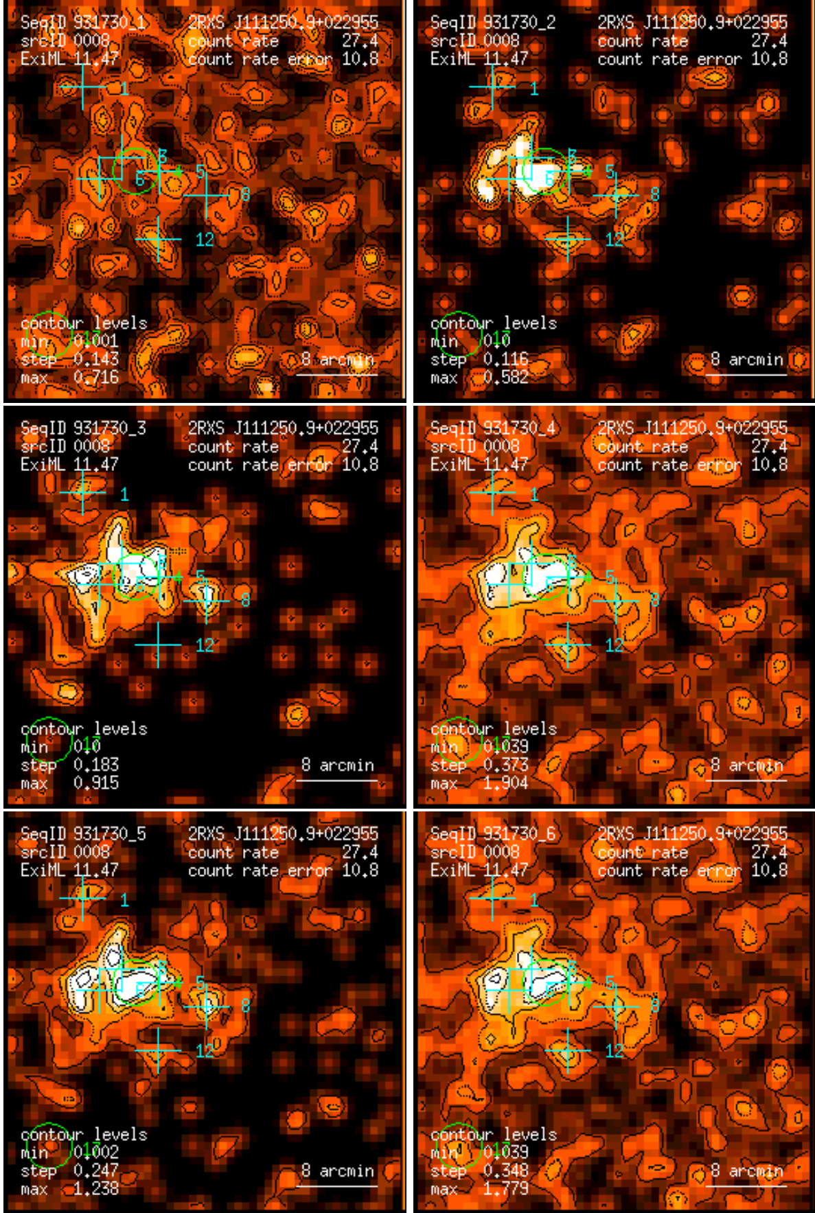
Figure 8: RASS 931730: detection 0008: band rate images, Gaussian filter: (1) PSPC channels 11 – 41, (2) 52 – 90, (3) 91 – 201, (4) 11 – 235, (5) 52 – 201, (6) 11 – 201. Broad band rates in counts/ks. Band rate contour levels in counts/ks/arcmin 2 .
