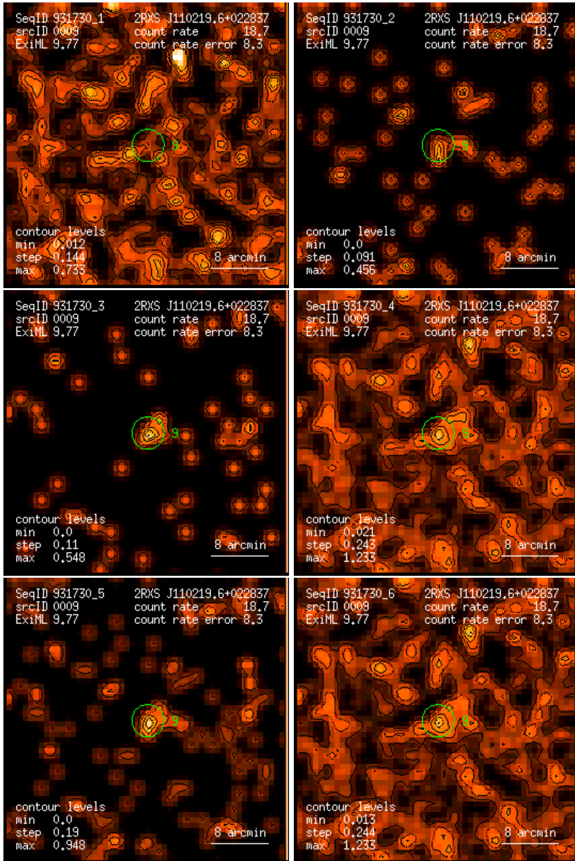
Figure 9: RASS 931730: detection 0009: band rate images, Gaussian filter: (1) PSPC channels 11 – 41, (2) 52 – 90, (3) 91 – 201, (4) 11 – 235, (5) 52 – 201, (6) 11 – 201. Broad band rates in counts/ks. Band rate contour levels in counts/ks/arcmin 2 .
