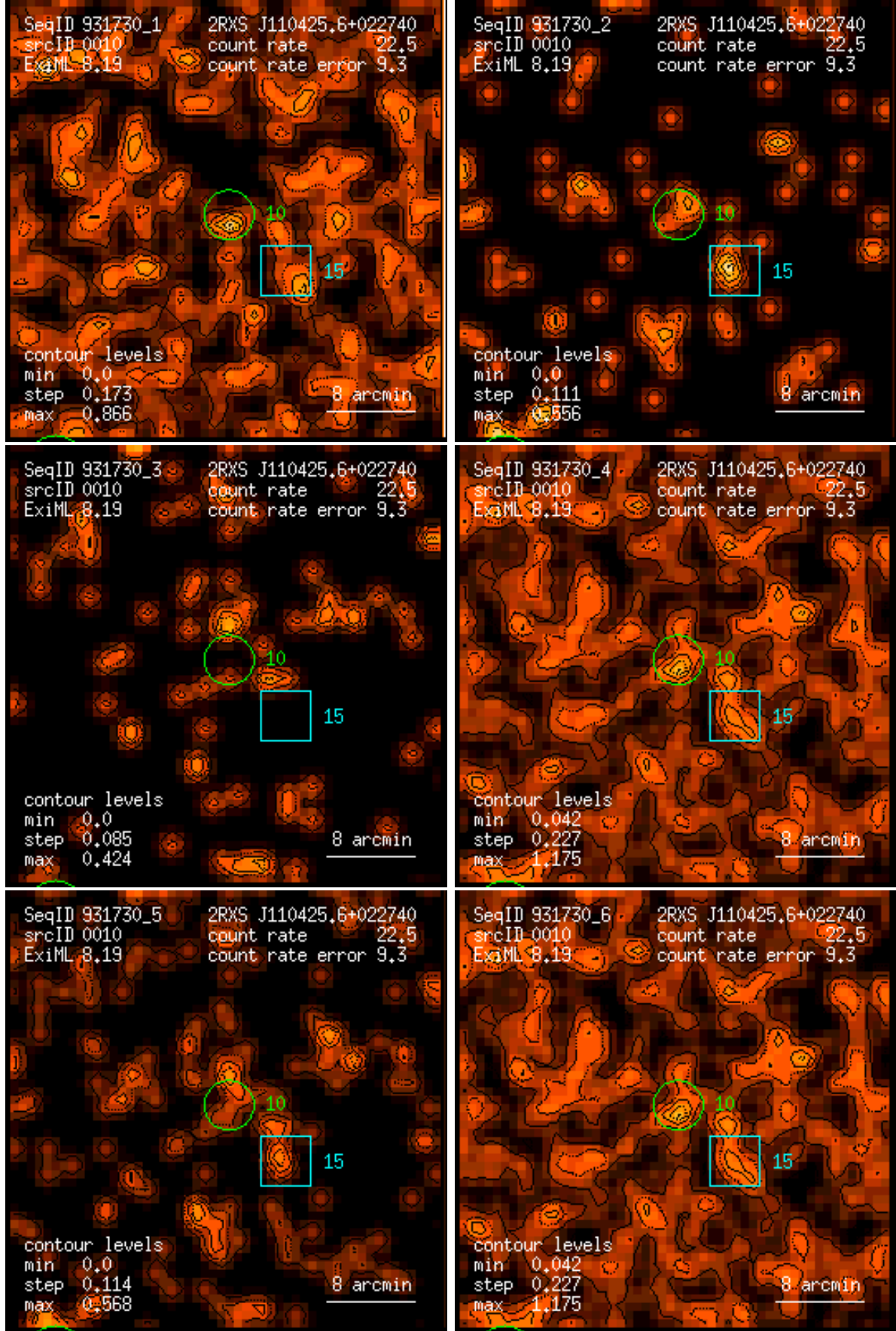
Figure 10: RASS 931730: detection 0010: band rate images, Gaussian filter: (1) PSPC channels 11 – 41, (2) 52 – 90, (3) 91 – 201, (4) 11 – 235, (5) 52 – 201, (6) 11 – 201. Broad band rates in counts/ks. Band rate contour levels in counts/ks/arcmin 2 .
