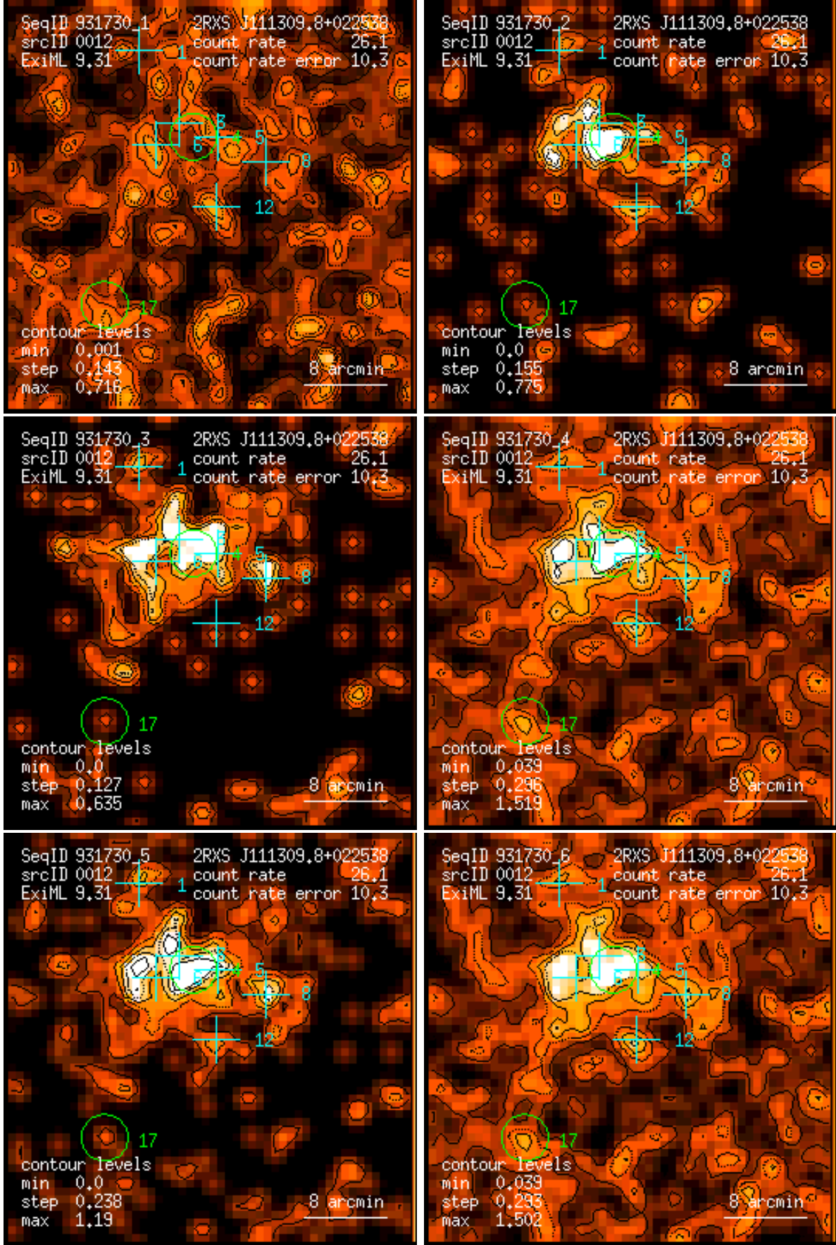
Figure 12: RASS 931730: detection 0012: band rate images, Gaussian filter: (1) PSPC channels 11 – 41, (2) 52 – 90, (3) 91 – 201, (4) 11 – 235, (5) 52 – 201, (6) 11 – 201. Broad band rates in counts/ks. Band rate contour levels in counts/ks/arcmin 2 .
