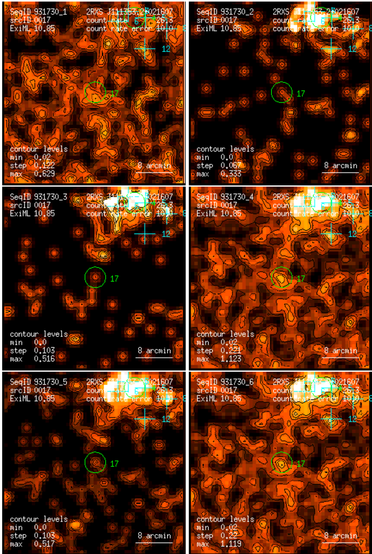
Figure 17: RASS 931730: detection 0017: band rate images, Gaussian filter: (1) PSPC channels 11 – 41, (2) 52 – 90, (3) 91 – 201, (4) 11 – 235, (5) 52 – 201, (6) 11 – 201. Broad band rates in counts/ks. Band rate contour levels in counts/ks/arcmin 2 .
