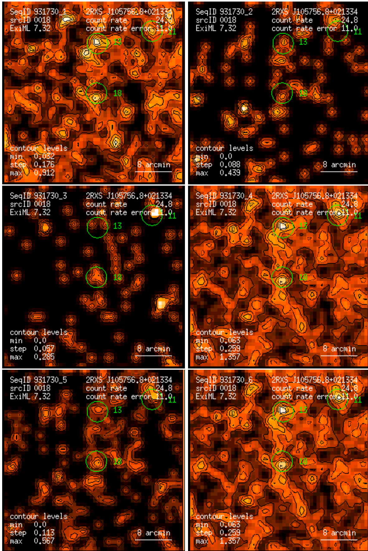
Figure 18: RASS 931730: detection 0018: band rate images, Gaussian filter: (1) PSPC channels 11 – 41, (2) 52 – 90, (3) 91 – 201, (4) 11 – 235, (5) 52 – 201, (6) 11 – 201. Broad band rates in counts/ks. Band rate contour levels in counts/ks/arcmin 2 .
