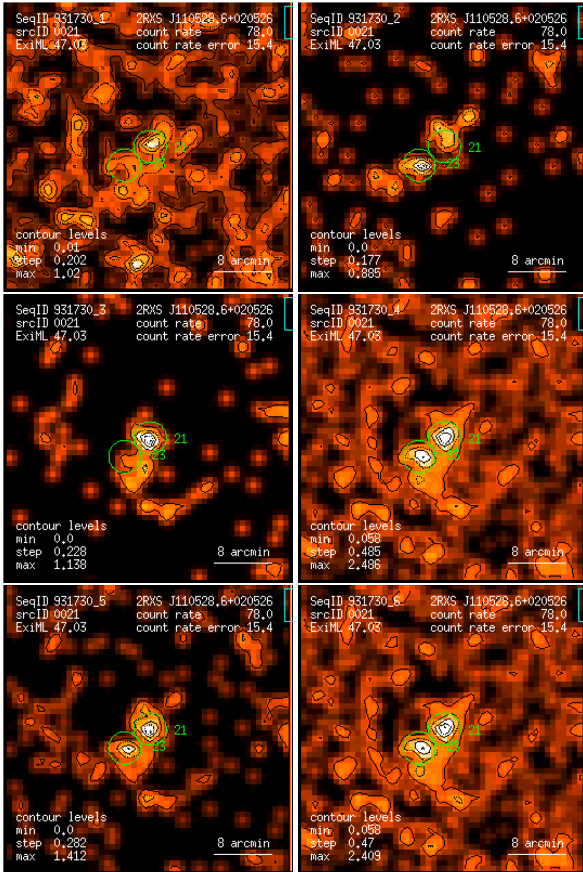
Figure 21: RASS 931730: detection 0021: band rate images, Gaussian filter: (1) PSPC channels 11 – 41, (2) 52 – 90, (3) 91 – 201, (4) 11 – 235, (5) 52 – 201, (6) 11 – 201. Broad band rates in counts/ks. Band rate contour levels in counts/ks/arcmin 2 .
