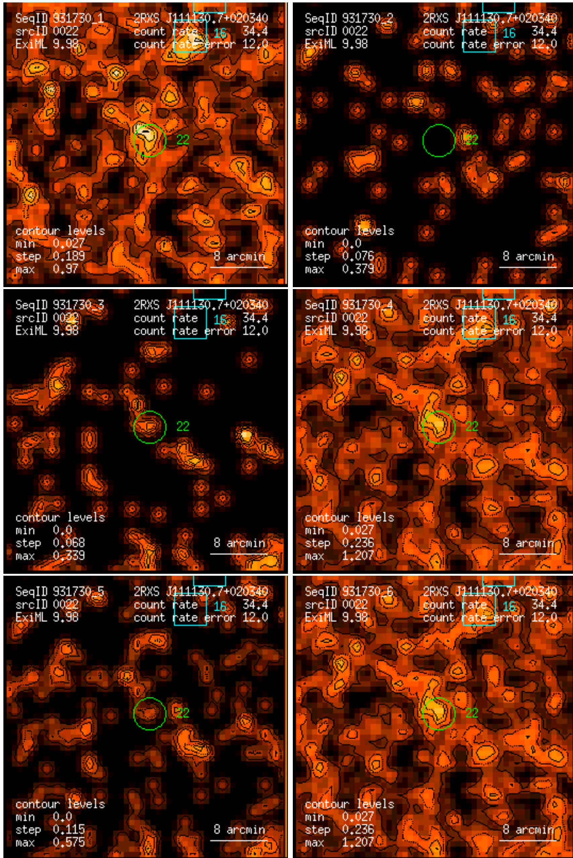
Figure 22: RASS 931730: detection 0022: band rate images, Gaussian filter: (1) PSPC channels 11 – 41, (2) 52 – 90, (3) 91 – 201, (4) 11 – 235, (5) 52 – 201, (6) 11 – 201. Broad band rates in counts/ks. Band rate contour levels in counts/ks/arcmin 2 .
