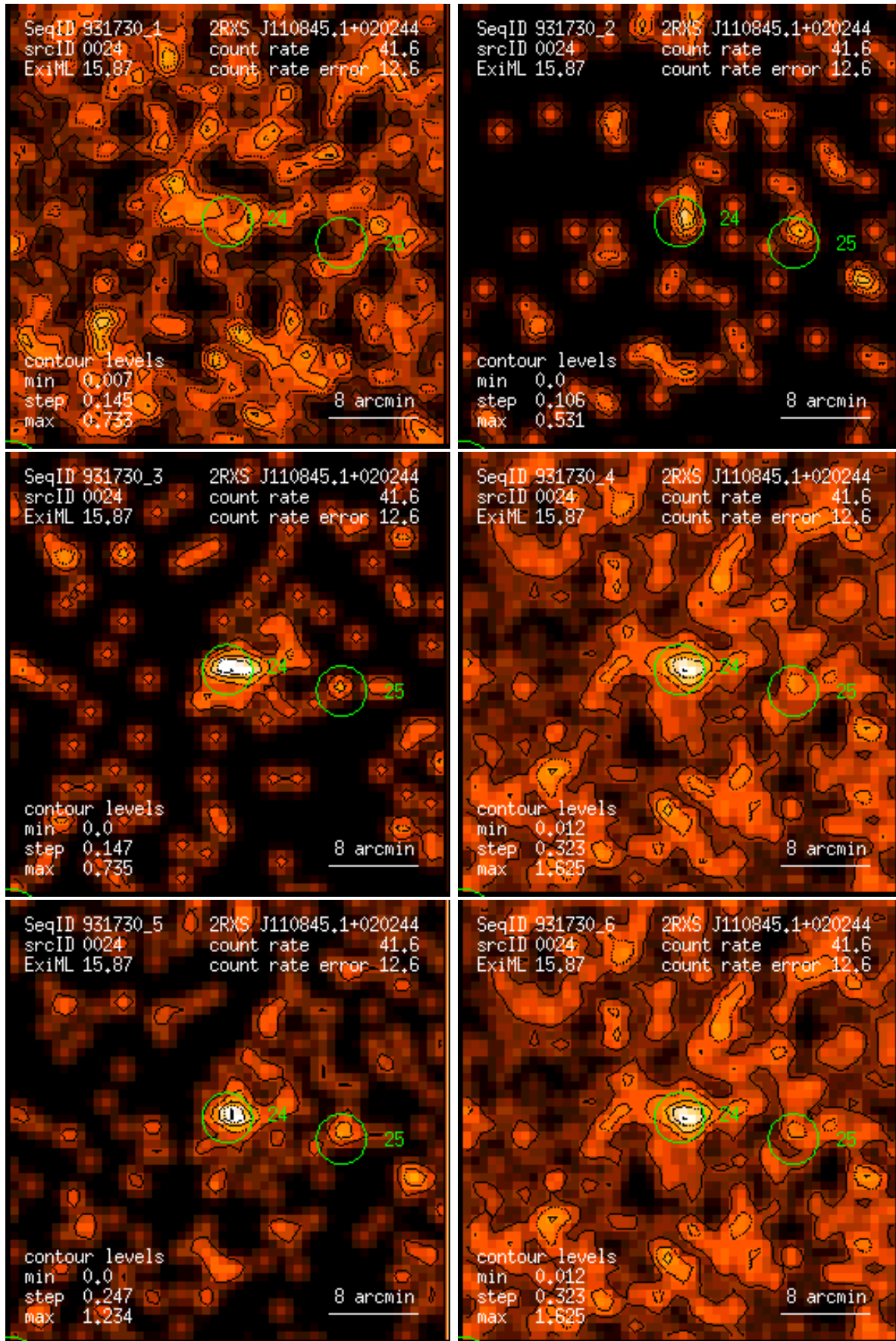
Figure 24: RASS 931730: detection 0024: band rate images, Gaussian filter: (1) PSPC channels 11 – 41, (2) 52 – 90, (3) 91 – 201, (4) 11 – 235, (5) 52 – 201, (6) 11 – 201. Broad band rates in counts/ks. Band rate contour levels in counts/ks/arcmin 2 .
