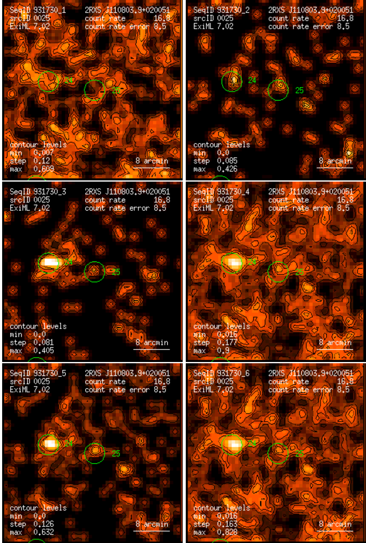
Figure 25: RASS 931730: detection 0025: band rate images, Gaussian filter: (1) PSPC channels 11 – 41, (2) 52 – 90, (3) 91 – 201, (4) 11 – 235, (5) 52 – 201, (6) 11 – 201. Broad band rates in counts/ks. Band rate contour levels in counts/ks/arcmin 2 .
