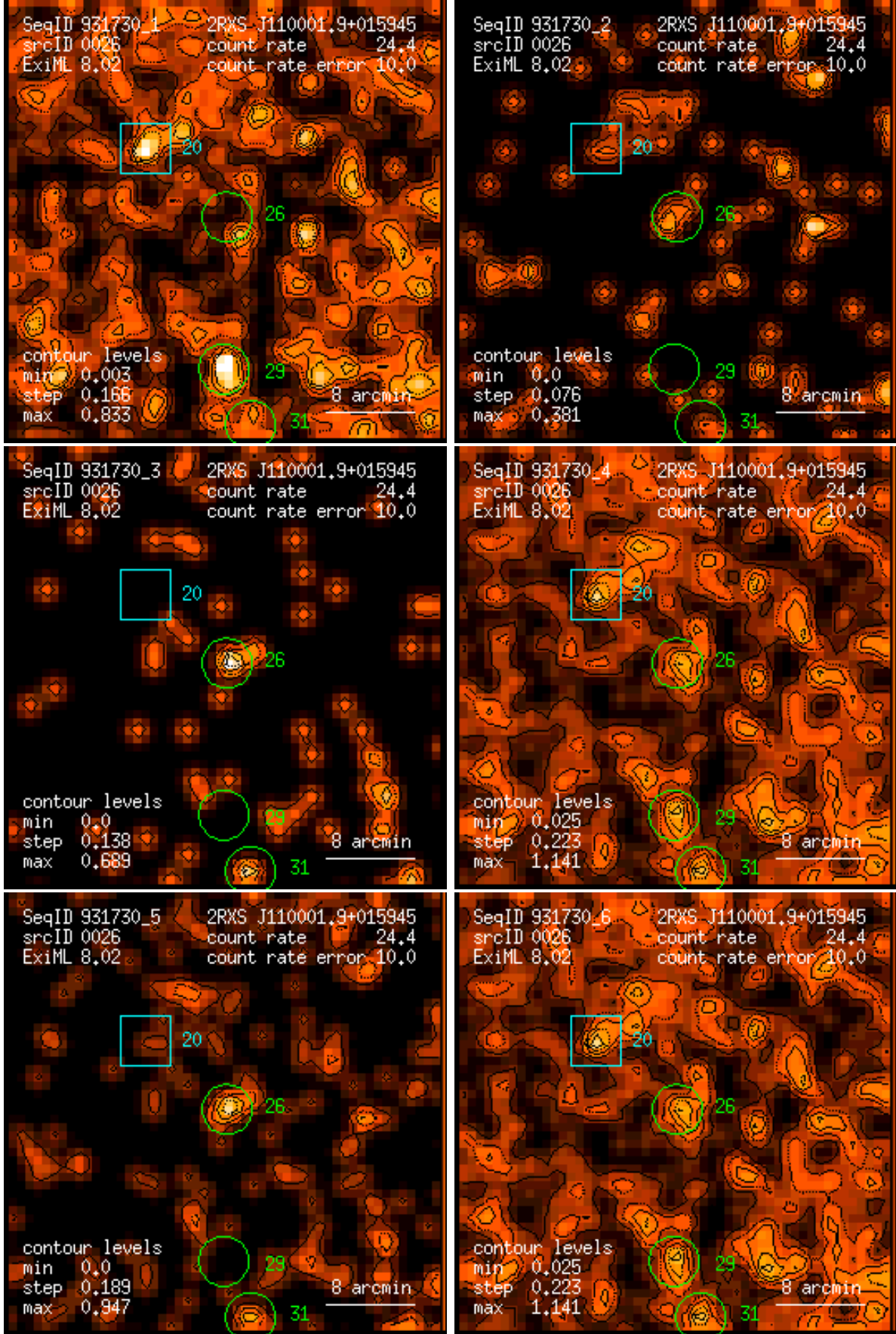
Figure 26: RASS 931730: detection 0026: band rate images, Gaussian filter: (1) PSPC channels 11 – 41, (2) 52 – 90, (3) 91 – 201, (4) 11 – 235, (5) 52 – 201, (6) 11 – 201. Broad band rates in counts/ks. Band rate contour levels in counts/ks/arcmin 2 .
