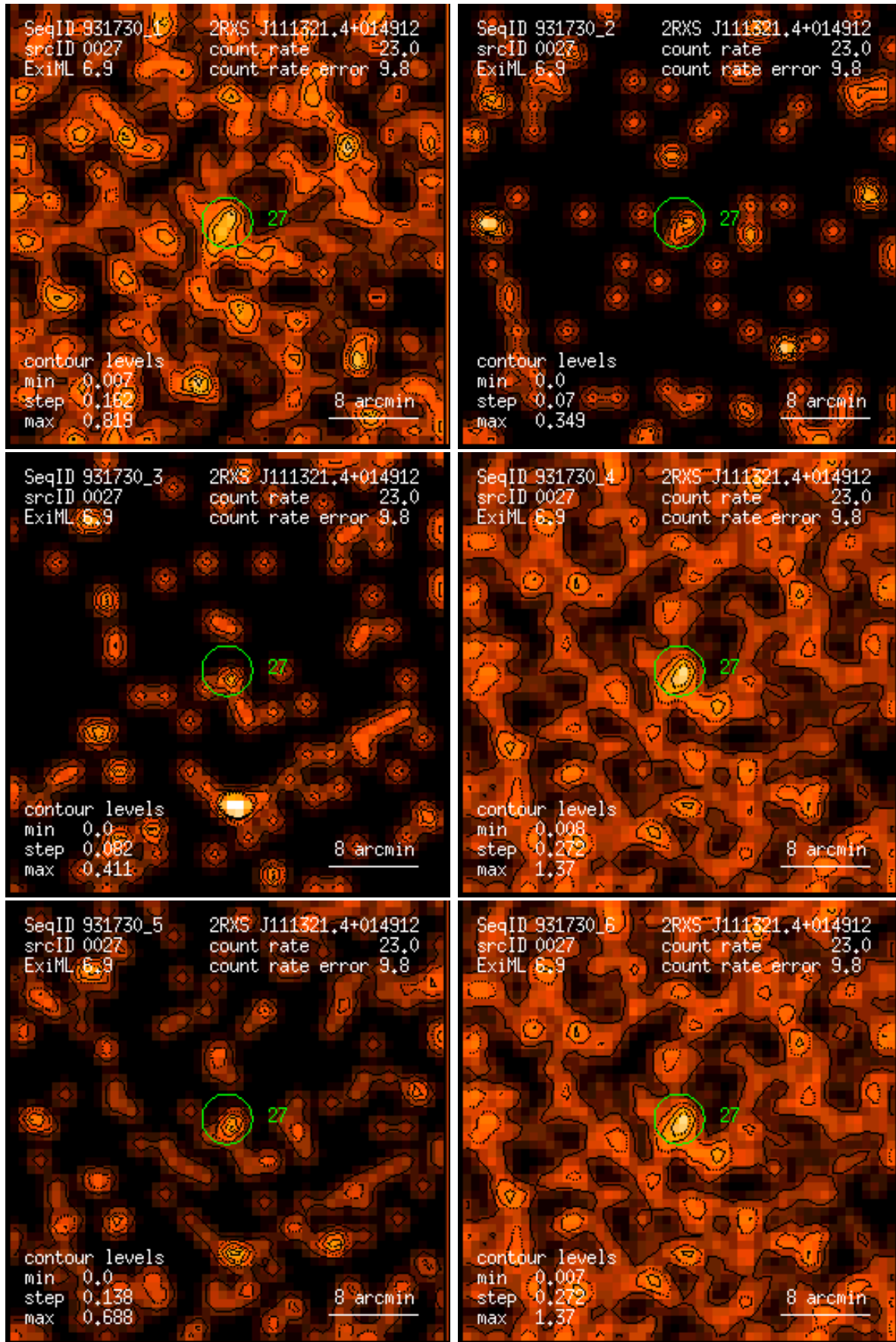
Figure 27: RASS 931730: detection 0027: band rate images, Gaussian filter: (1) PSPC channels 11 – 41, (2) 52 – 90, (3) 91 – 201, (4) 11 – 235, (5) 52 – 201, (6) 11 – 201. Broad band rates in counts/ks. Band rate contour levels in counts/ks/arcmin 2 .
