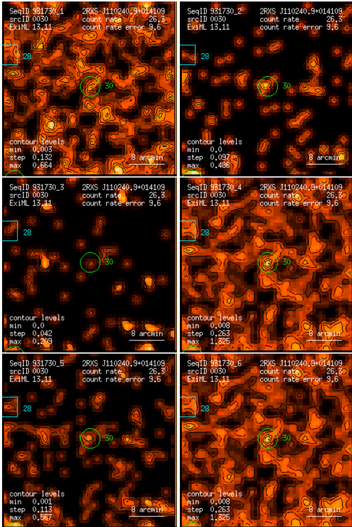
Figure 30: RASS 931730: detection 0030: band rate images, Gaussian filter: (1) PSPC channels 11 – 41, (2) 52 – 90, (3) 91 – 201, (4) 11 – 235, (5) 52 – 201, (6) 11 – 201. Broad band rates in counts/ks. Band rate contour levels in counts/ks/arcmin 2 .
