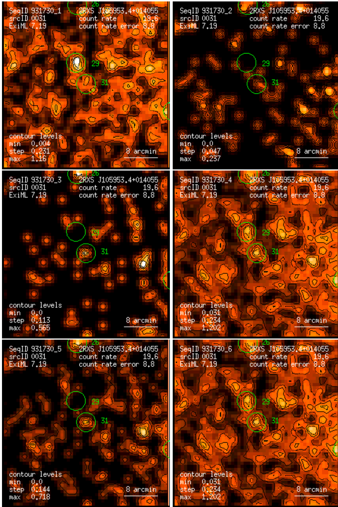
Figure 31: RASS 931730: detection 0031: band rate images, Gaussian filter: (1) PSPC channels 11 – 41, (2) 52 – 90, (3) 91 – 201, (4) 11 – 235, (5) 52 – 201, (6) 11 – 201. Broad band rates in counts/ks. Band rate contour levels in counts/ks/arcmin 2 .
