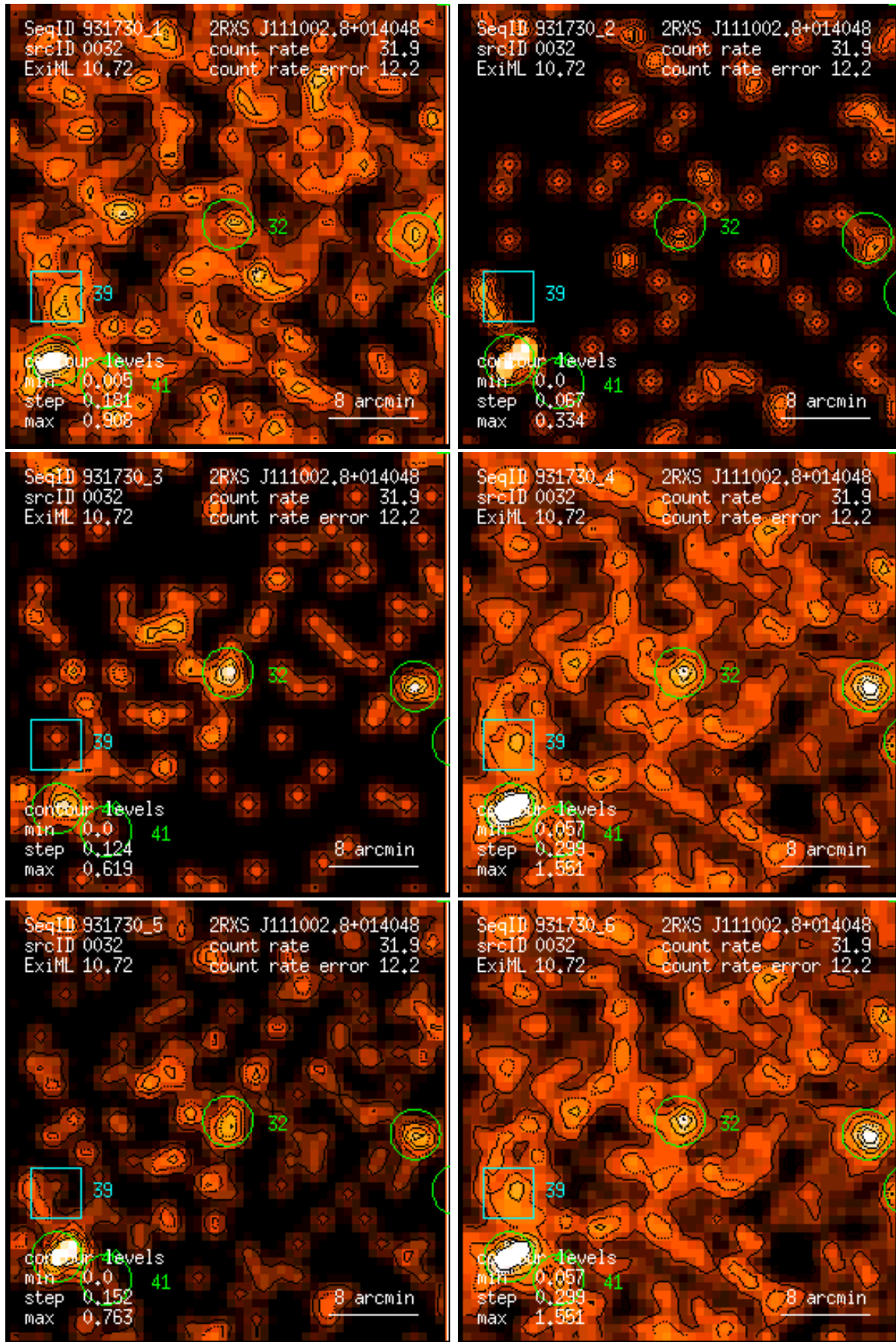
Figure 32: RASS 931730: detection 0032: band rate images, Gaussian filter: (1) PSPC channels 11 – 41, (2) 52 – 90, (3) 91 – 201, (4) 11 – 235, (5) 52 – 201, (6) 11 – 201. Broad band rates in counts/ks. Band rate contour levels in counts/ks/arcmin 2 .
