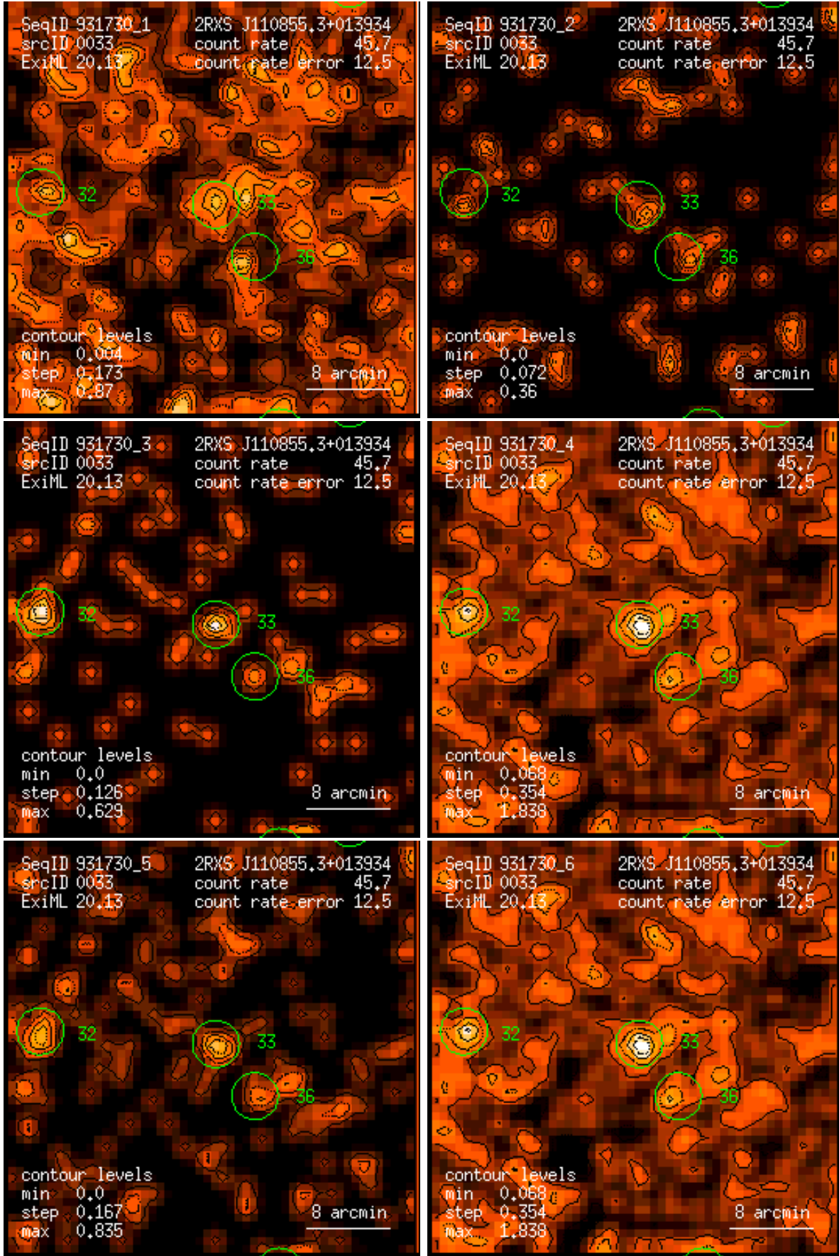
Figure 33: RASS 931730: detection 0033: band rate images, Gaussian filter: (1) PSPC channels 11 – 41, (2) 52 – 90, (3) 91 – 201, (4) 11 – 235, (5) 52 – 201, (6) 11 – 201. Broad band rates in counts/ks. Band rate contour levels in counts/ks/arcmin 2 .
