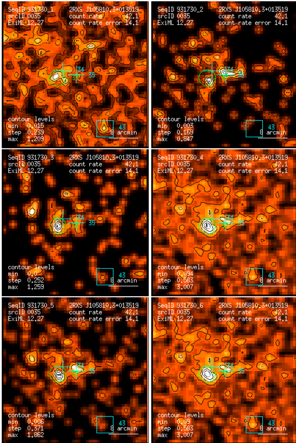
Figure 35: RASS 931730: detection 0035: band rate images, Gaussian filter: (1) PSPC channels 11 – 41, (2) 52 – 90, (3) 91 – 201, (4) 11 – 235, (5) 52 – 201, (6) 11 – 201. Broad band rates in counts/ks. Band rate contour levels in counts/ks/arcmin 2 .
