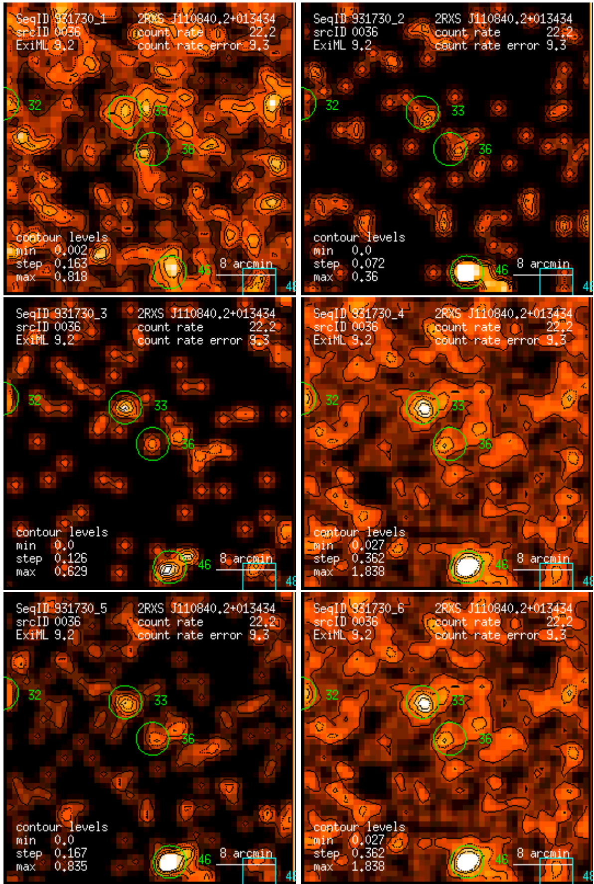
Figure 36: RASS 931730: detection 0036: band rate images, Gaussian filter: (1) PSPPC channels 11 – 41, (2) 52 – 90, (3) 91 – 201, (4) 11 – 235, (5) 52 – 201, (6) 11 – 201. Broad band rates in counts/ks. Band rate contour levels in counts/ks/arcmin 2 .
