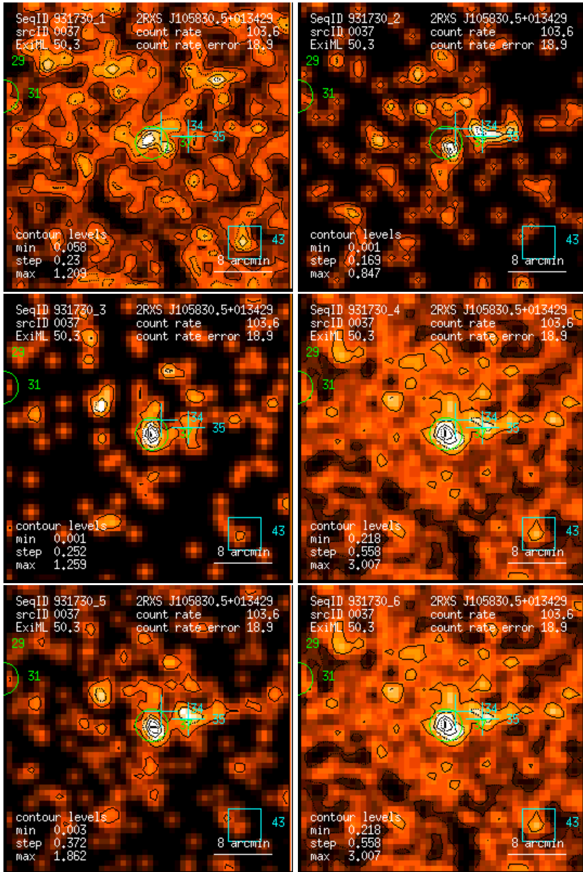
Figure 37: RASS 931730: detection 0037: band rate images, Gaussian filter: (1) PSPC channels 11 – 41, (2) 52 – 90, (3) 91 – 201, (4) 11 – 235, (5) 52 – 201, (6) 11 – 201. Broad band rates in counts/ks. Band rate contour levels in counts/ks/arcmin 2 .
