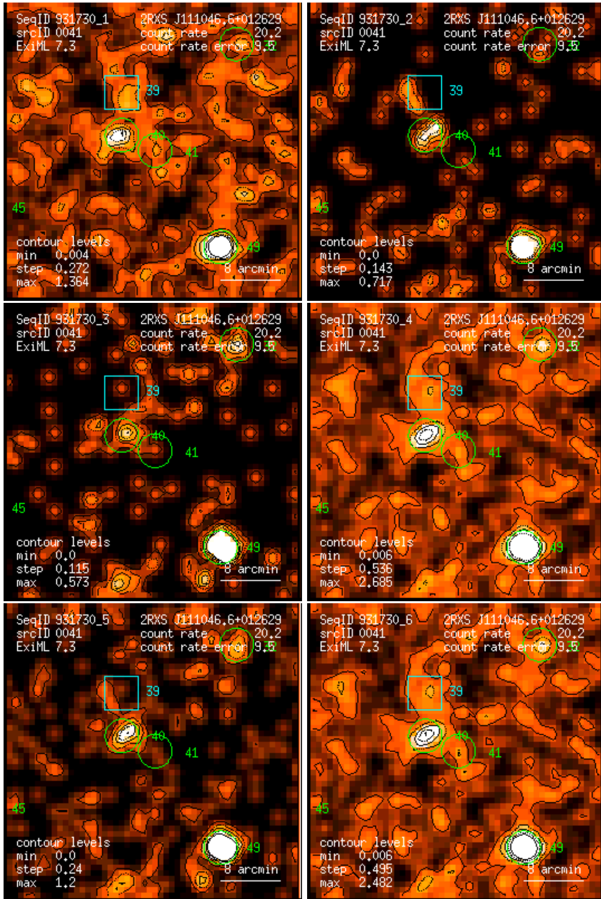
Figure 41: RASS 931730: detection 0041: band rate images, Gaussian filter: (1) PSPC channels 11 – 41, (2) 52 – 90, (3) 91 – 201, (4) 11 – 235, (5) 52 – 201, (6) 11 – 201. Broad band rates in counts/ks. Band rate contour levels in counts/ks/arcmin 2 .
