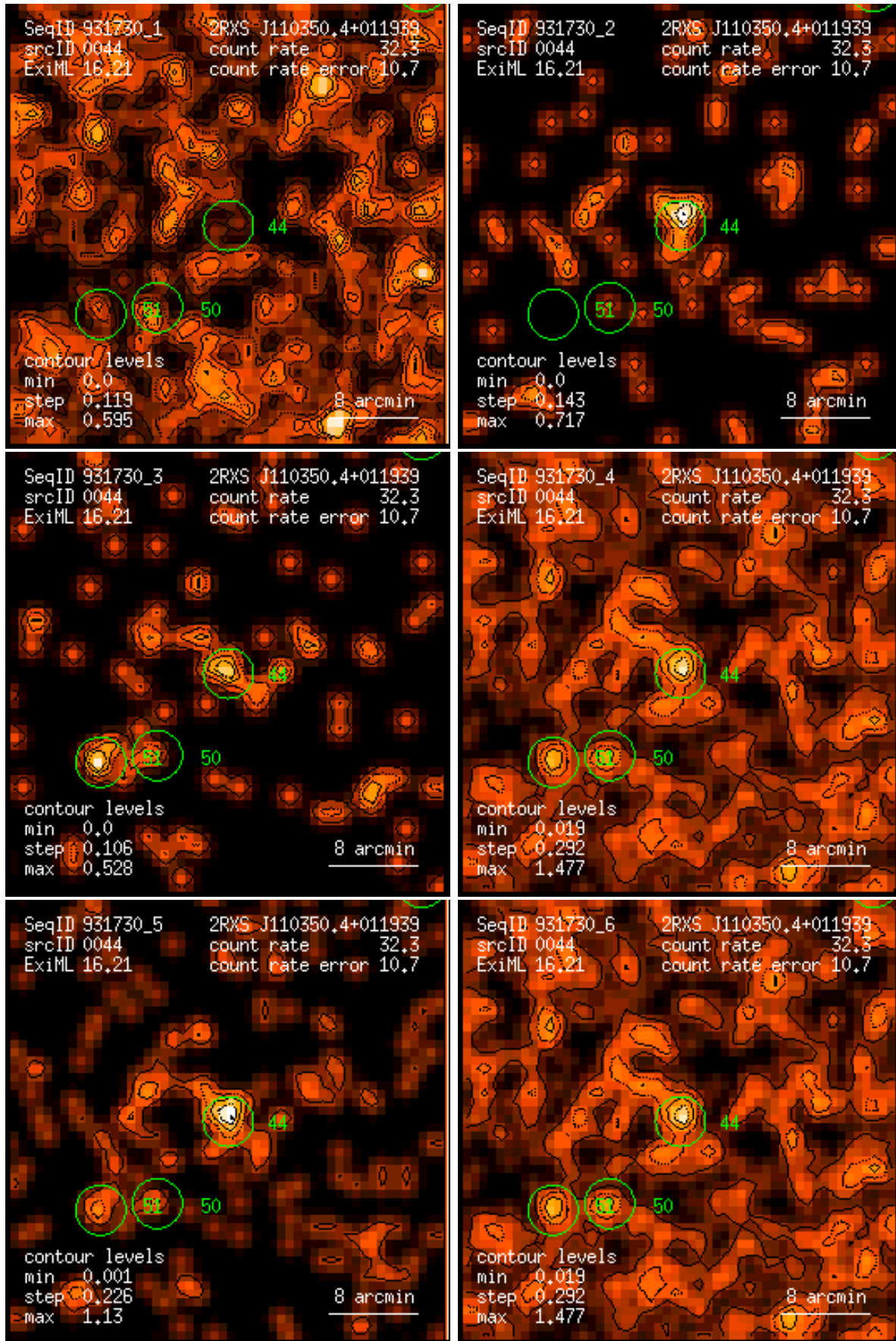
Figure 44: RASS 931730: detection 0044: band rate images, Gaussian filter: (1) PSPC channels 11 – 41, (2) 52 – 90, (3) 91 – 201, (4) 11 – 235, (5) 52 – 201, (6) 11 – 201. Broad band rates in counts/ks. Band rate contour levels in counts/ks/arcmin 2 .
