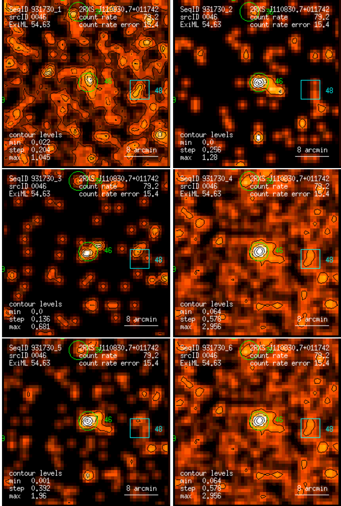
Figure 46: RASS 931730: detection 0046: band rate images, Gaussian filter: (1) PSPC channels 11 – 41, (2) 52 – 90, (3) 91 – 201, (4) 11 – 235, (5) 52 – 201, (6) 11 – 201. Broad band rates in counts/ks. Band rate contour levels in counts/ks/arcmin 2 .
